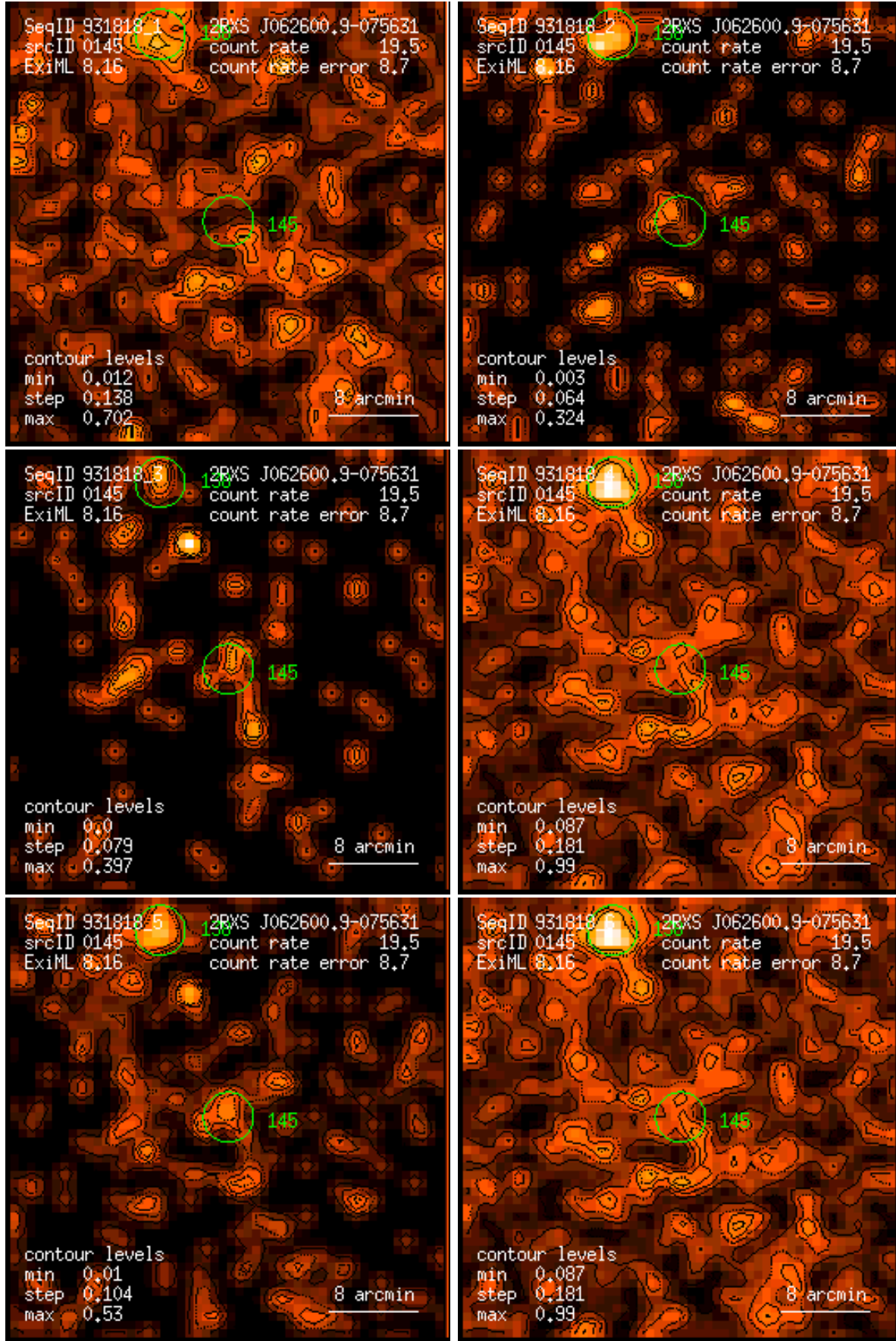
Figure 145: RASS 931818: detection 0145: band rate images, Gaussian filter: (1) PSPC channels 11 – 41, (2) 52 – 90, (3) 91 – 201, (4) 11 – 235, (5) 52 – 201, (6) 11 – 201. Broad band rates in counts/ks. Band rate contour levels in counts/ks/arcmin 2 .
