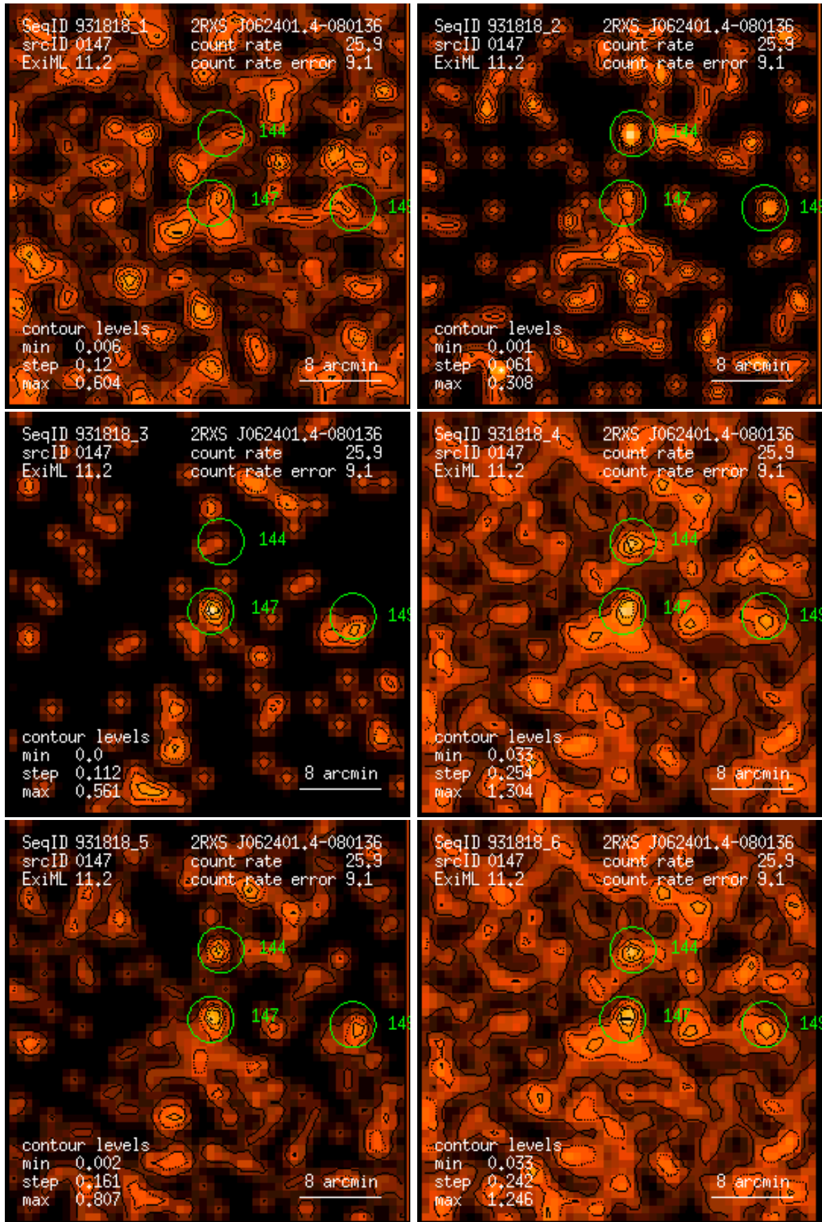
Figure 147: RASS 931818: detection 0147: band rate images, Gaussian filter: (1) PSPC channels 11 – 41, (2) 52 – 90, (3) 91 – 201, (4) 11 – 235, (5) 52 – 201, (6) 11 – 201. Broad band rates in counts/ks. Band rate contour levels in counts/ks/arcmin 2 .
