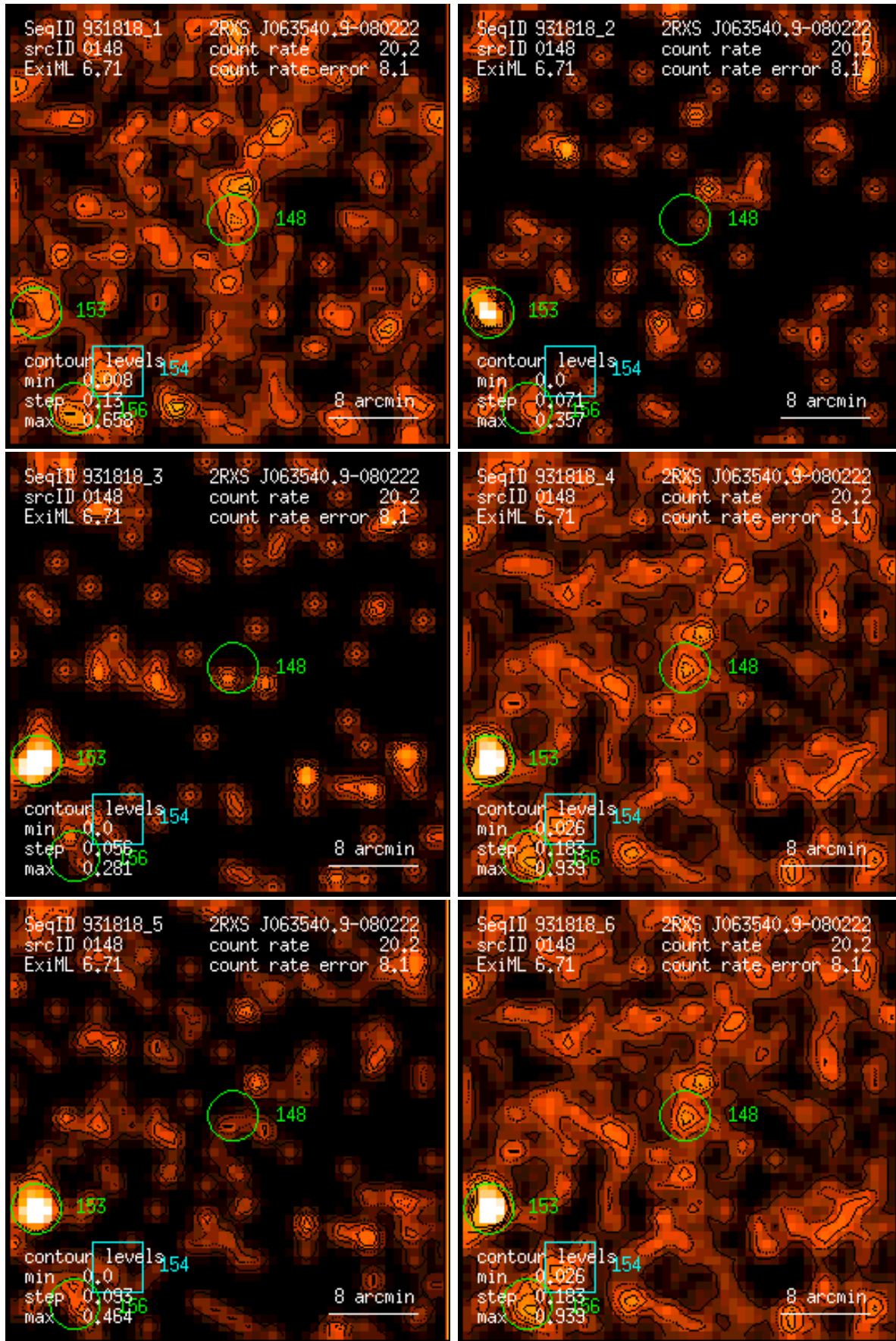
Figure 148: RASS 931818: detection 0148: band rate images, Gaussian filter: (1) PSPC channels 11 – 41, (2) 52 – 90, (3) 91 – 201, (4) 11 – 235, (5) 52 – 201, (6) 11 – 201. Broad band rates in counts/ks. Band rate contour levels in counts/ks/arcmin 2 .
