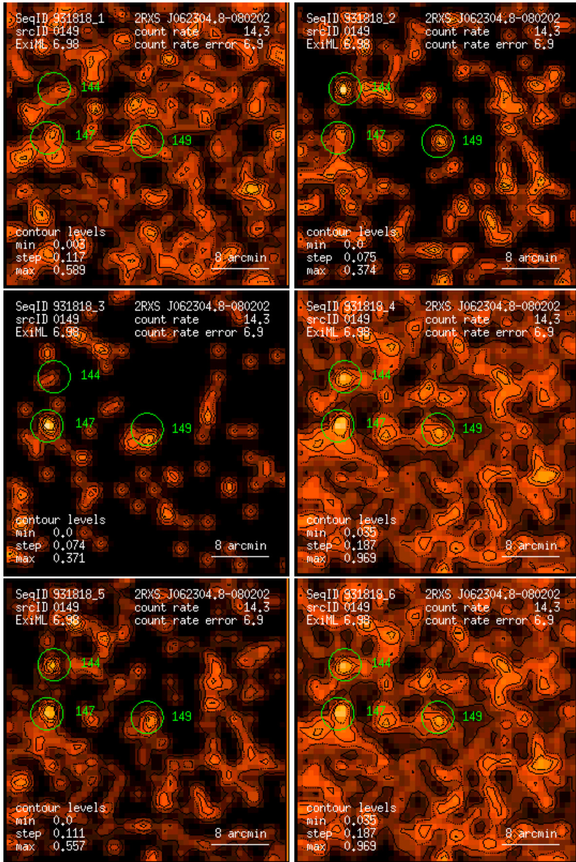
Figure 149: RASS 931818: detection 0149: band rate images, Gaussian filter: (1) PSPC channels 11 – 41, (2) 52 – 90, (3) 91 – 201, (4) 11 – 235, (5) 52 – 201, (6) 11 – 201. Broad band rates in counts/ks. Band rate contour levels in counts/ks/arcmin 2 .
