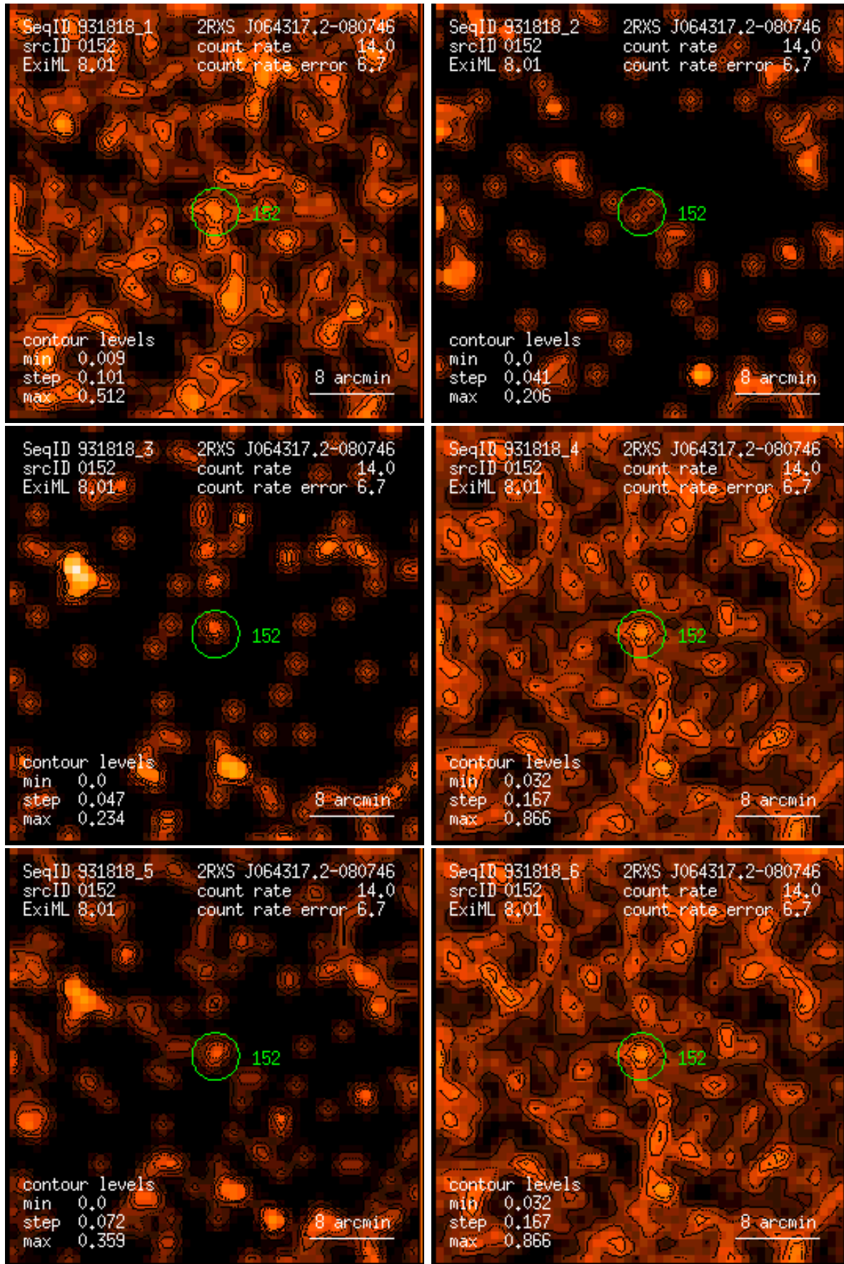
Figure 152: RASS 931818: detection 0152: band rate images, Gaussian filter: (1) PSPC channels 11 – 41, (2) 52 – 90, (3) 91 – 201, (4) 11 – 235, (5) 52 – 201, (6) 11 – 201. Broad band rates in counts/ks. Band rate contour levels in counts/ks/arcmin 2 .
