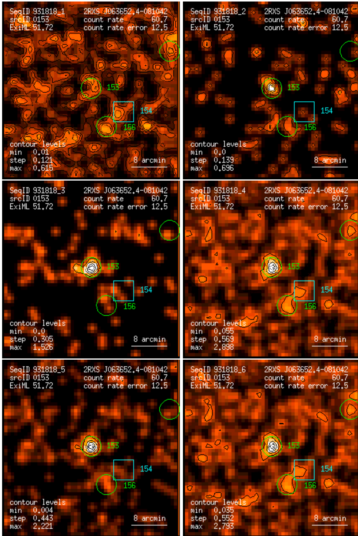
Figure 153: RASS 931818: detection 0153: band rate images, Gaussian filter: (1) PSPC channels 11 – 41, (2) 52 – 90, (3) 91 – 201, (4) 11 – 235, (5) 52 – 201, (6) 11 – 201. Broad band rates in counts/ks. Band rate contour levels in counts/ks/arcmin 2 .
