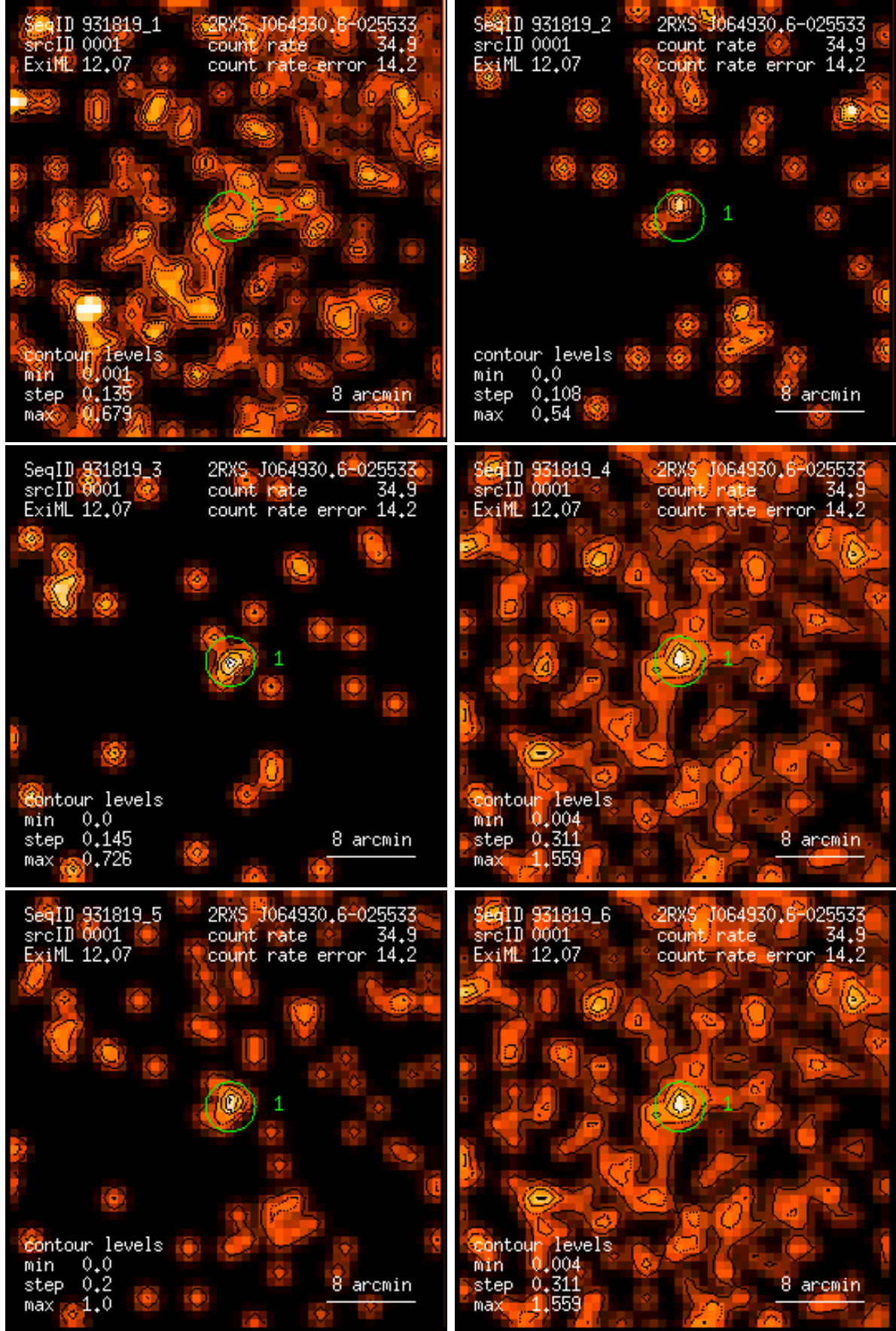
Figure 1: RASS 931819: detection 0001: band rate images, Gaussian filter: (1) PSPC channels 11 – 41, (2) 52 – 90, (3) 91 – 201, (4) 11 – 235, (5) 52 – 201, (6) 11 – 201. Broad band rates in counts/ks. Band rate contour levels in counts/ks/arcmin 2 .
