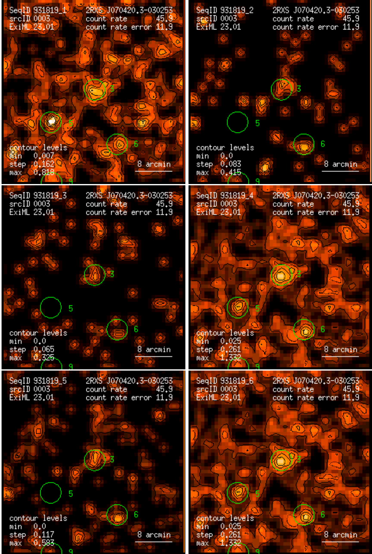
Figure 3: RASS 931819: detection 0003: band rate images, Gaussian filter: (1) PSPC channels 11 – 41, (2) 52 – 90, (3) 91 – 201, (4) 11 – 235, (5) 52 – 201, (6) 11 – 201. Broad band rates in counts/ks. Band rate contour levels in counts/ks/arcmin 2 .
