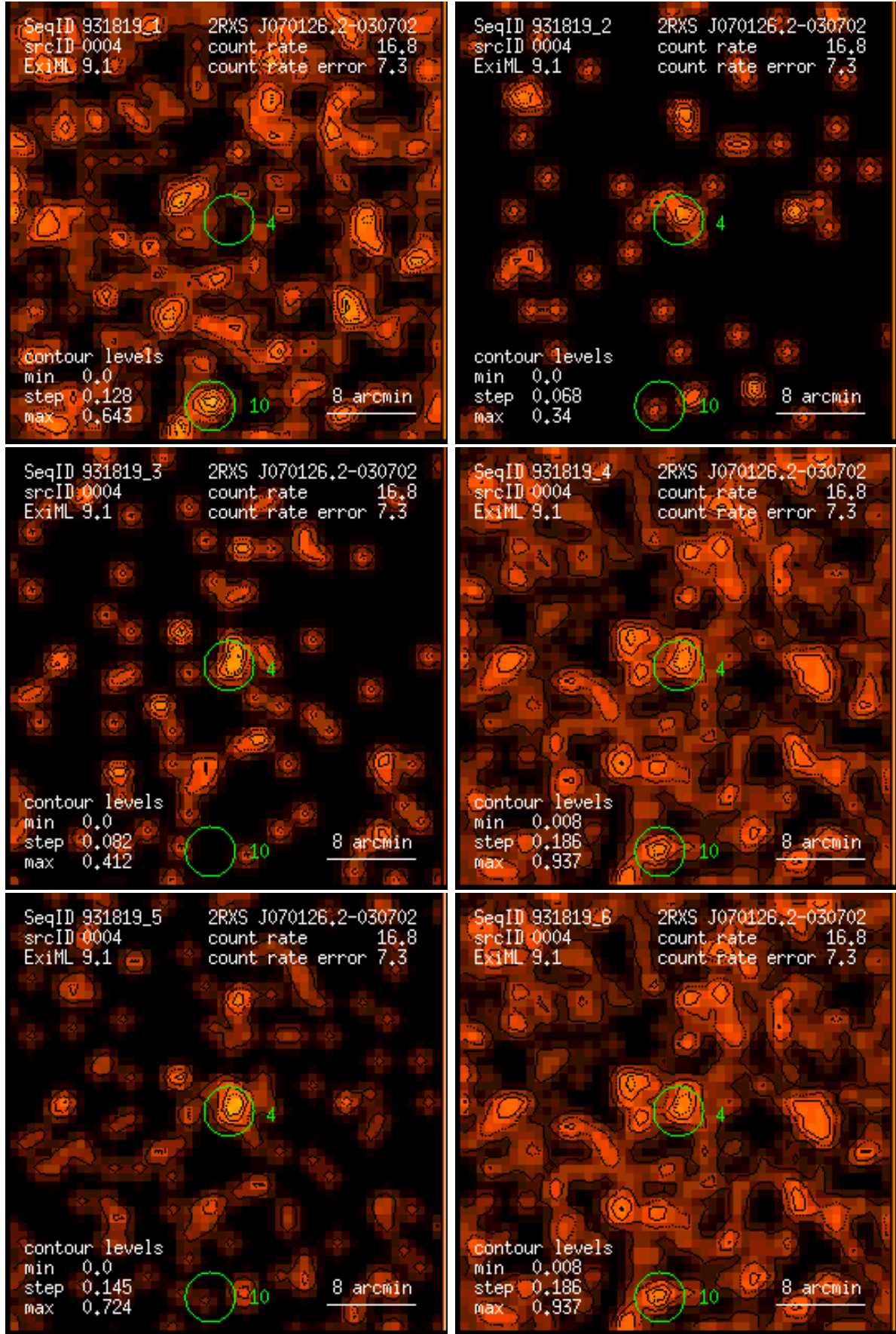
Figure 4: RASS 931819: detection 0004: band rate images, Gaussian filter: (1) PSPC channels 11 – 41, (2) 52 – 90, (3) 91 – 201, (4) 11 – 235, (5) 52 – 201, (6) 11 – 201. Broad band rates in counts/ks. Band rate contour levels in counts/ks/arcmin 2 .
