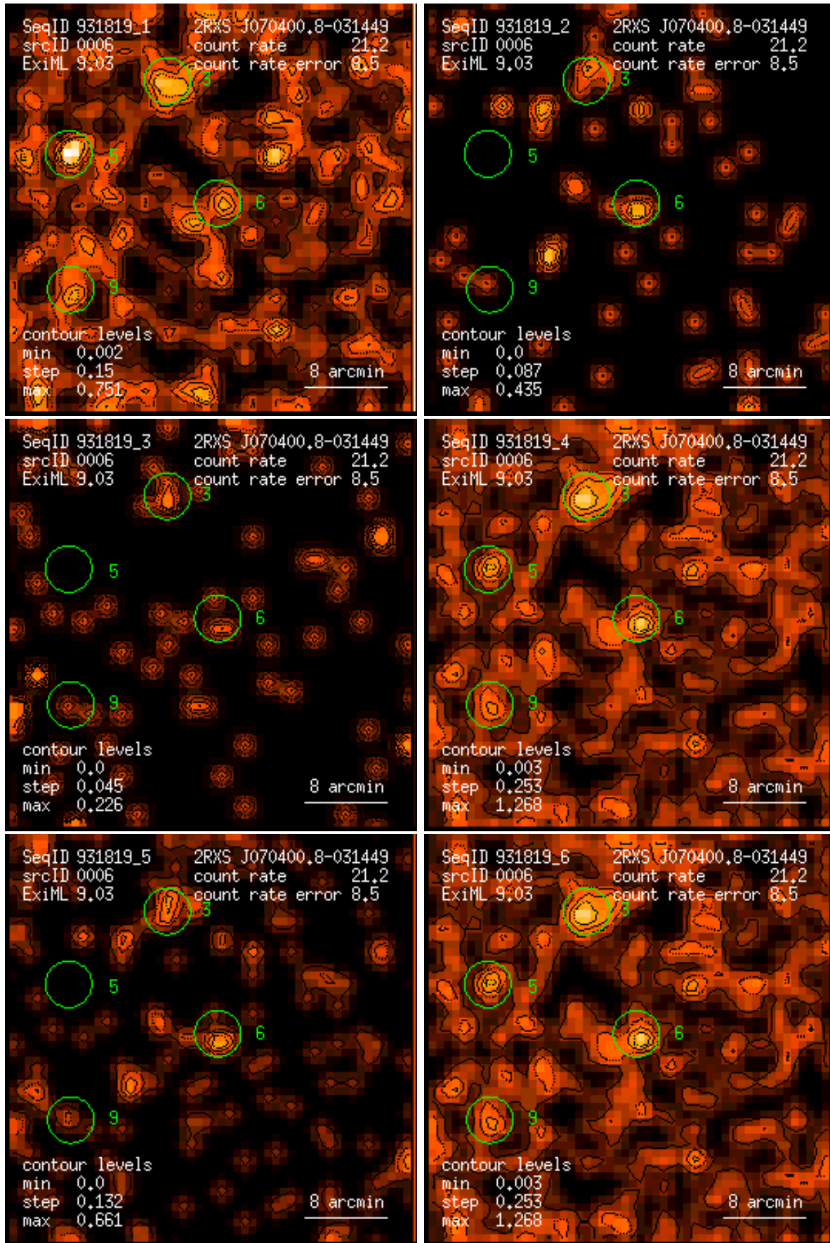
Figure 6: RASS 931819: detection 0006: band rate images, Gaussian filter: (1) PSPC channels 11 – 41, (2) 52 – 90, (3) 91 – 201, (4) 11 – 235, (5) 52 – 201, (6) 11 – 201. Broad band rates in counts/ks. Band rate contour levels in counts/ks/arcmin 2 .
