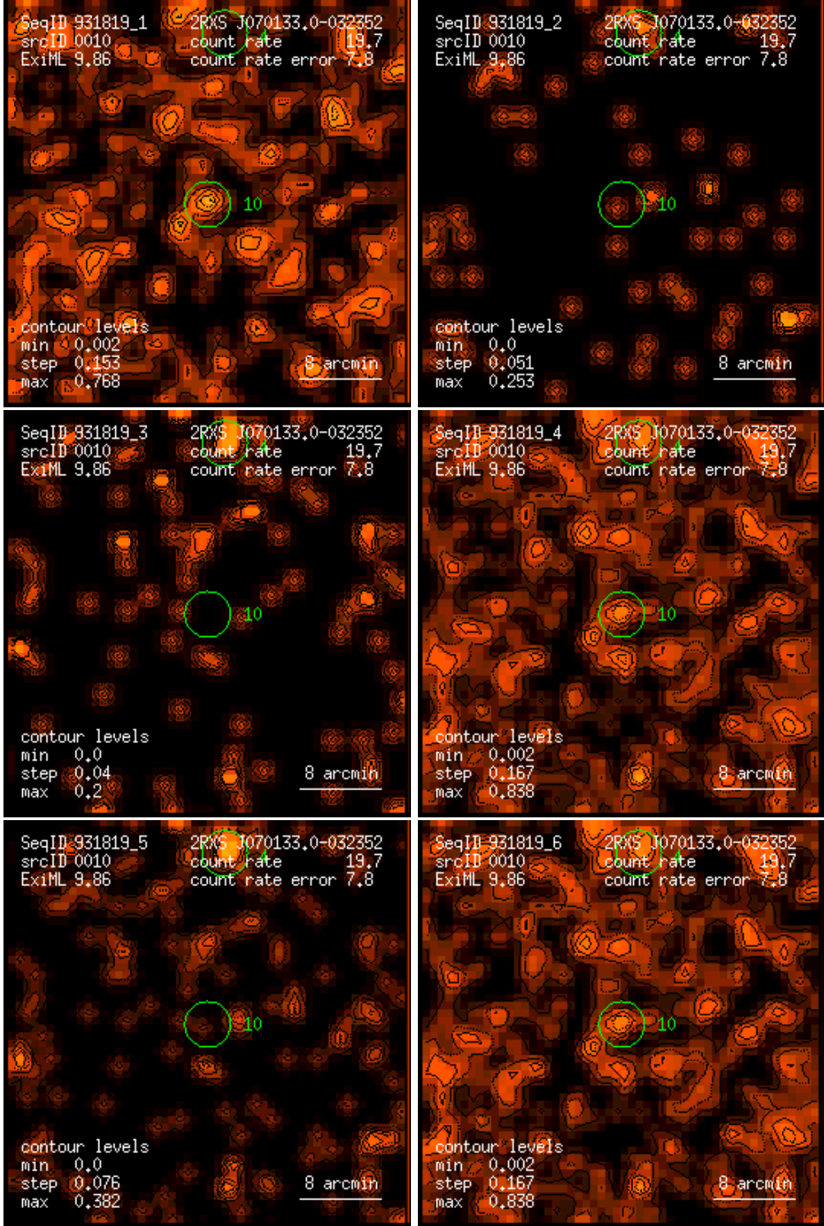
Figure 10: RASS 931819: detection 0010: band rate images, Gaussian filter: (1) PSPC channels 11 – 41, (2) 52 – 90, (3) 91 – 201, (4) 11 – 235, (5) 52 – 201, (6) 11 – 201. Broad band rates in counts/ks. Band rate contour levels in counts/ks/arcmin 2 .
