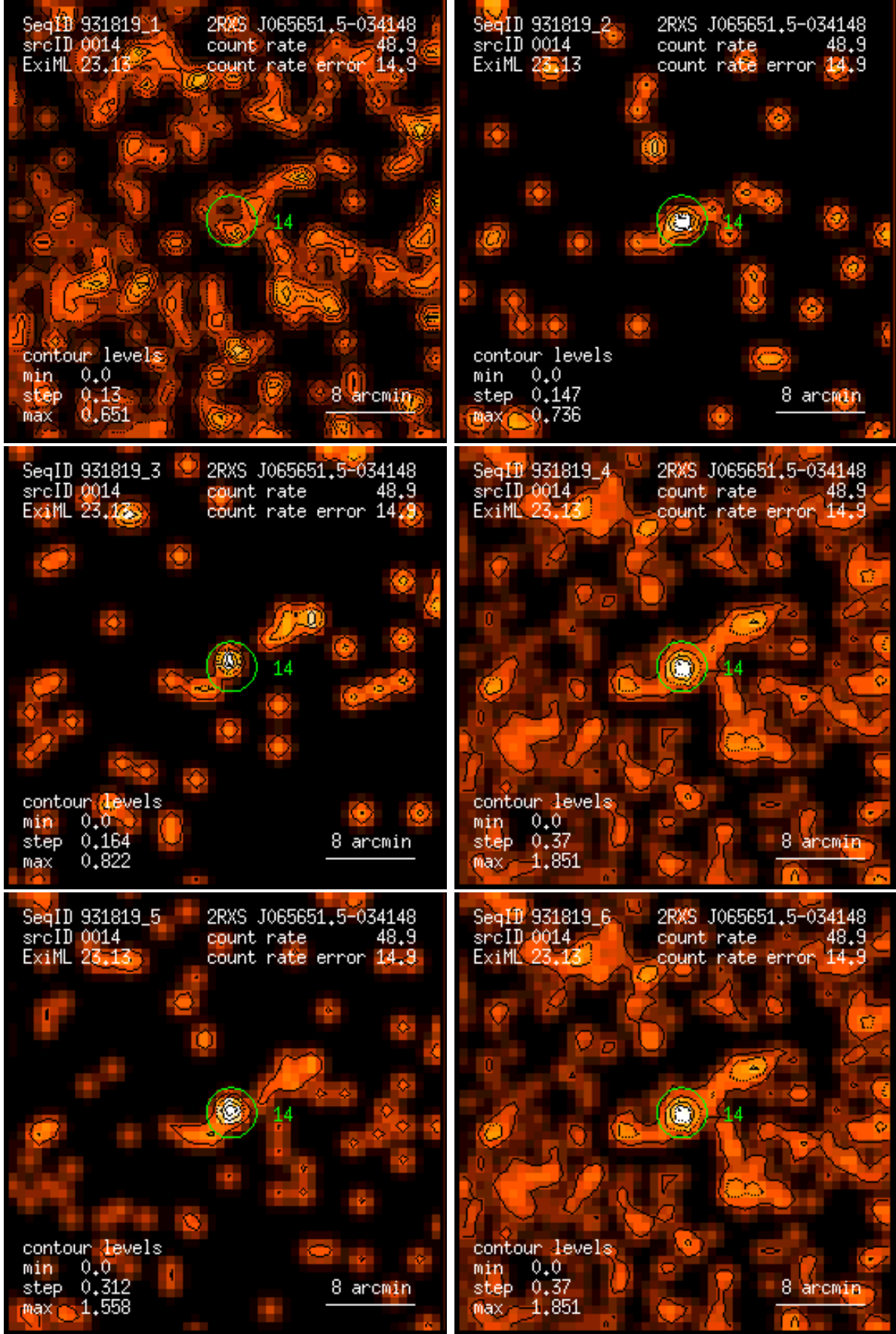
Figure 14: RASS 931819: detection 0014: band rate images, Gaussian filter: (1) PSPC channels 11 – 41, (2) 52 – 90, (3) 91 – 201, (4) 11 – 235, (5) 52 – 201, (6) 11 – 201. Broad band rates in counts/ks. Band rate contour levels in counts/ks/arcmin 2 .
