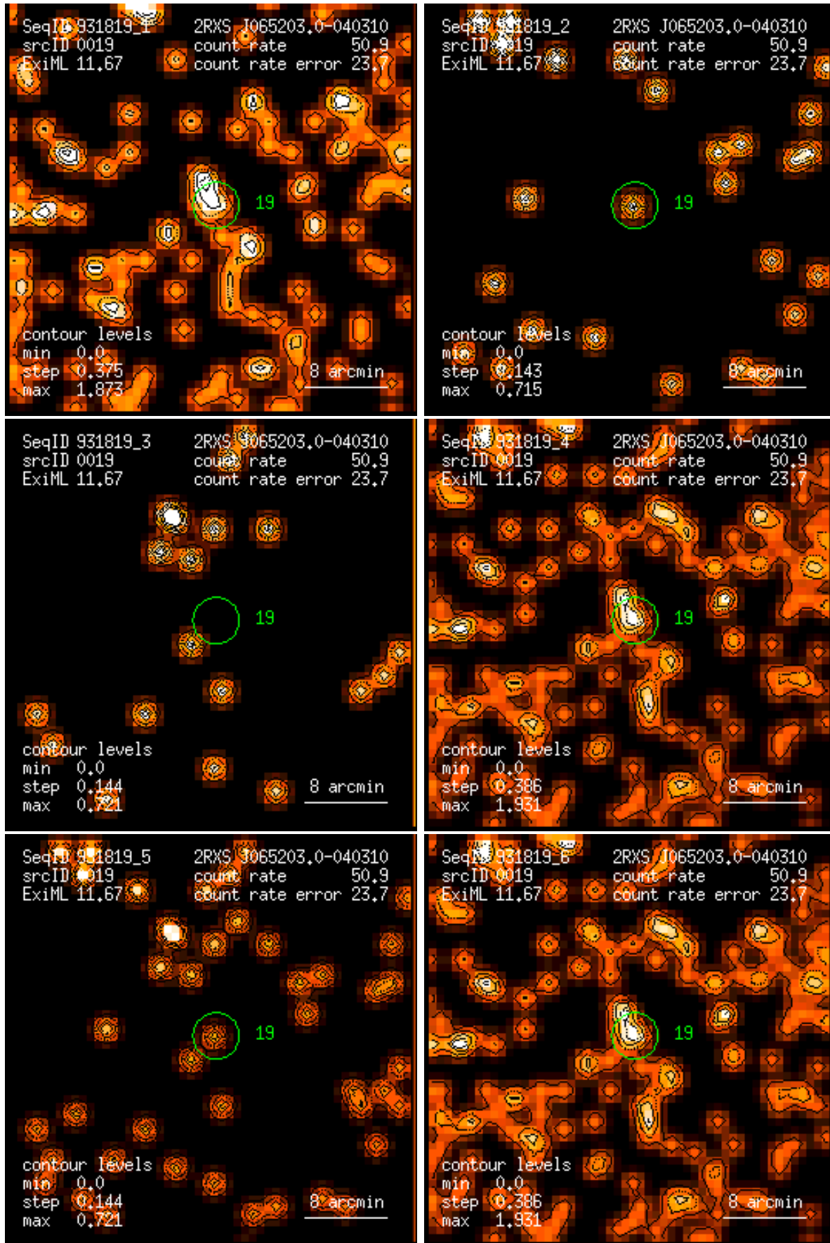
Figure 19: RASS 931819: detection 0019: band rate images, Gaussian filter: (1) PSPC channels 11 – 41, (2) 52 – 90, (3) 91 – 201, (4) 11 – 235, (5) 52 – 201, (6) 11 – 201. Broad band rates in counts/ks. Band rate contour levels in counts/ks/arcmin 2 .
