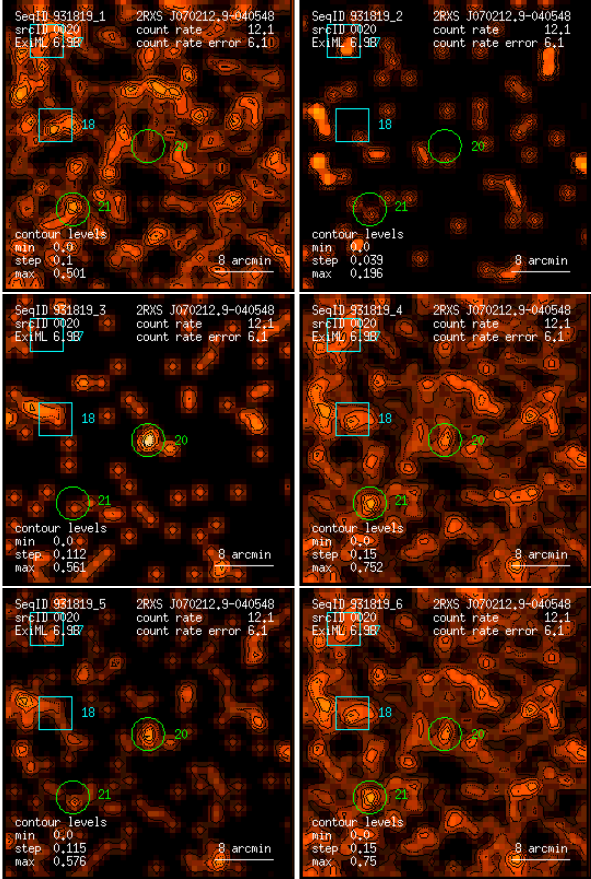
Figure 20: RASS 931819: detection 0020: band rate images, Gaussian filter: (1) PSPC channels 11 – 41, (2) 52 – 90, (3) 91 – 201, (4) 11 – 235, (5) 52 – 201, (6) 11 – 201. Broad band rates in counts/ks. Band rate contour levels in counts/ks/arcmin 2 .
