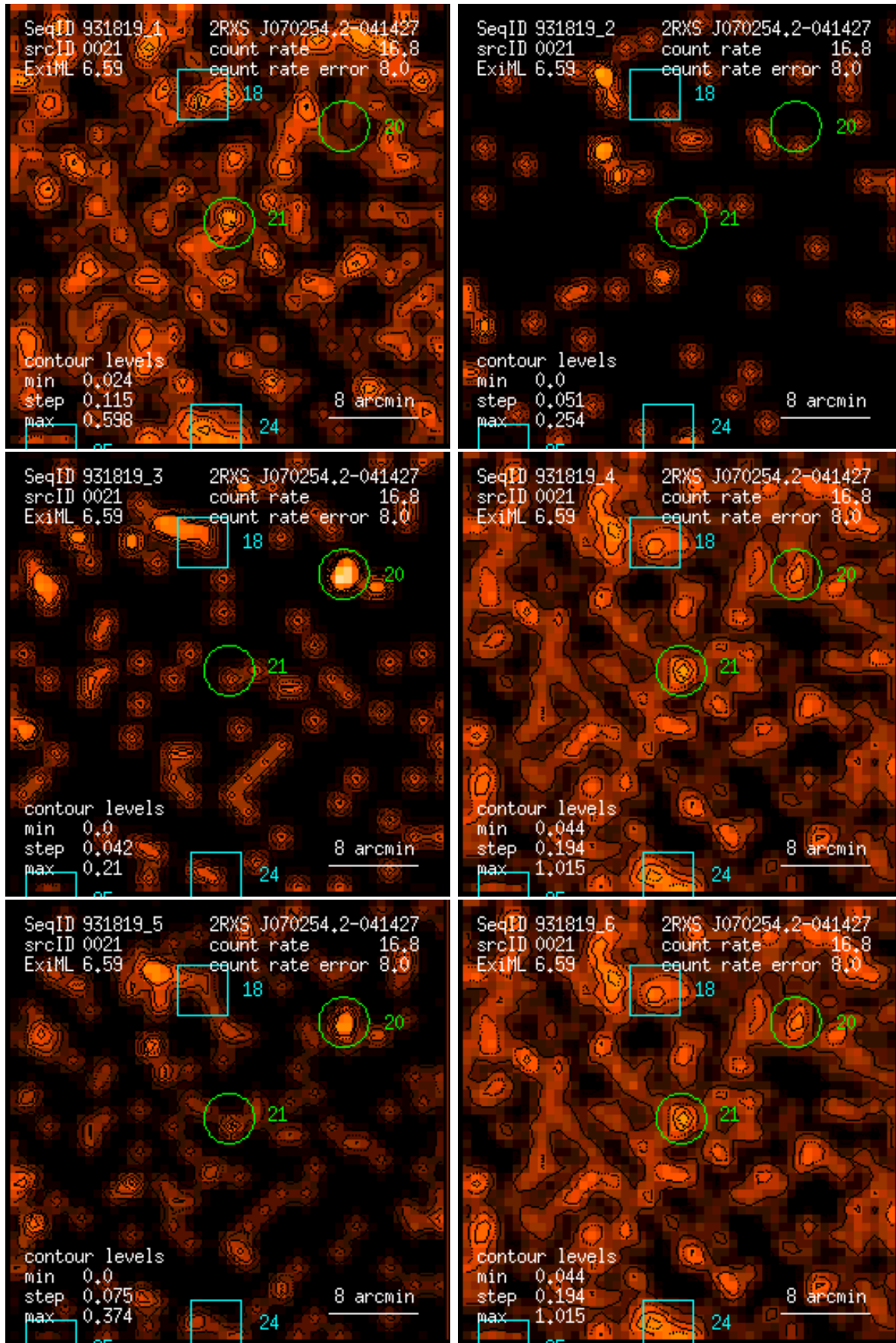
Figure 21: RASS 931819: detection 0021: band rate images, Gaussian filter: (1) PSPC channels 11 – 41, (2) 52 – 90, (3) 91 – 201, (4) 11 – 235, (5) 52 – 201, (6) 11 – 201. Broad band rates in counts/ks. Band rate contour levels in counts/ks/arcmin 2 .
