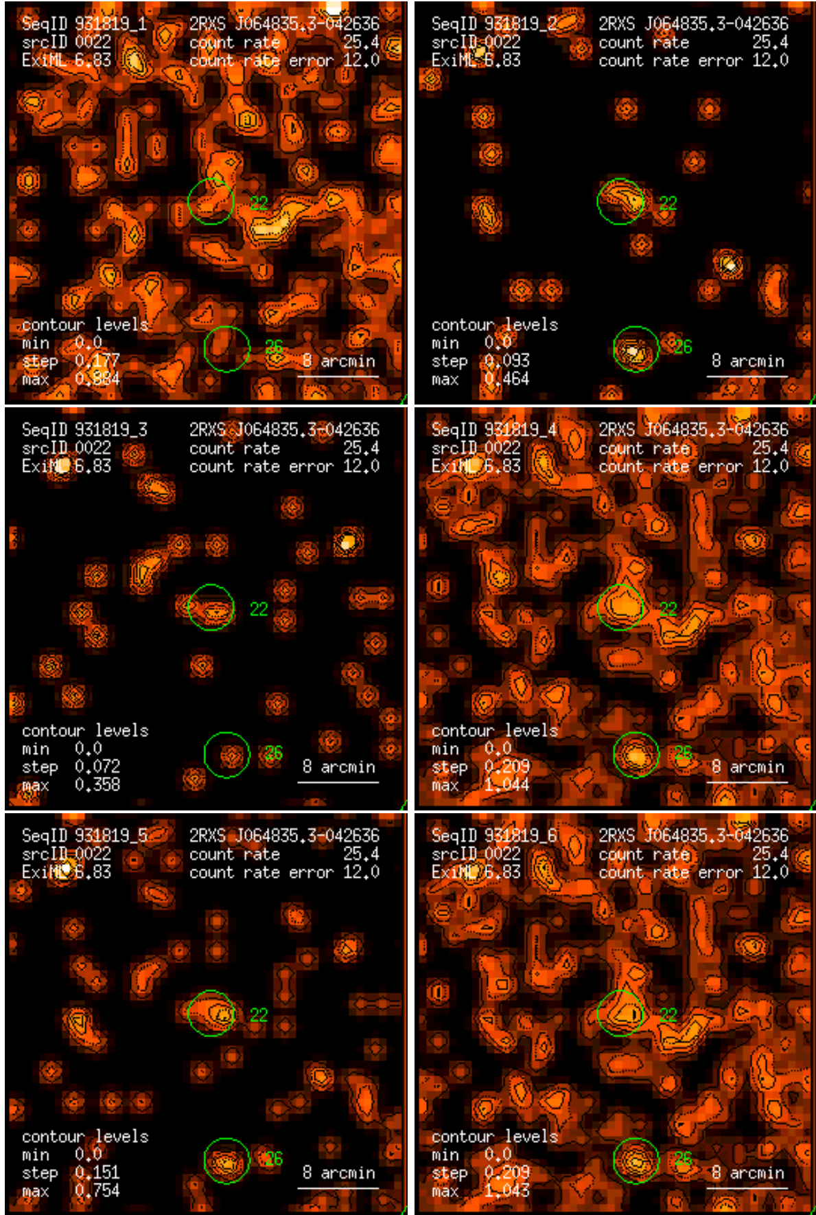
Figure 22: RASS 931819: detection 0022: band rate images, Gaussian filter: (1) PSPC channels 11 – 41, (2) 52 – 90, (3) 91 – 201, (4) 11 – 235, (5) 52 – 201, (6) 11 – 201. Broad band rates in counts/ks. Band rate contour levels in counts/ks/arcmin 2 .
