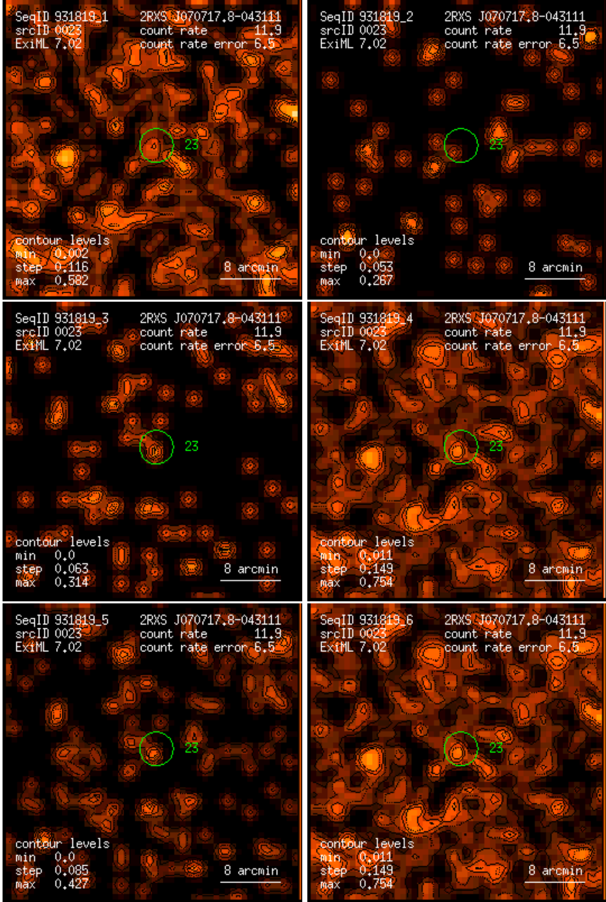
Figure 23: RASS 931819: detection 0023: band rate images, Gaussian filter: (1) PSPC channels 11 – 41, (2) 52 – 90, (3) 91 – 201, (4) 11 – 235, (5) 52 – 201, (6) 11 – 201. Broad band rates in counts/ks. Band rate contour levels in counts/ks/arcmin 2 .
