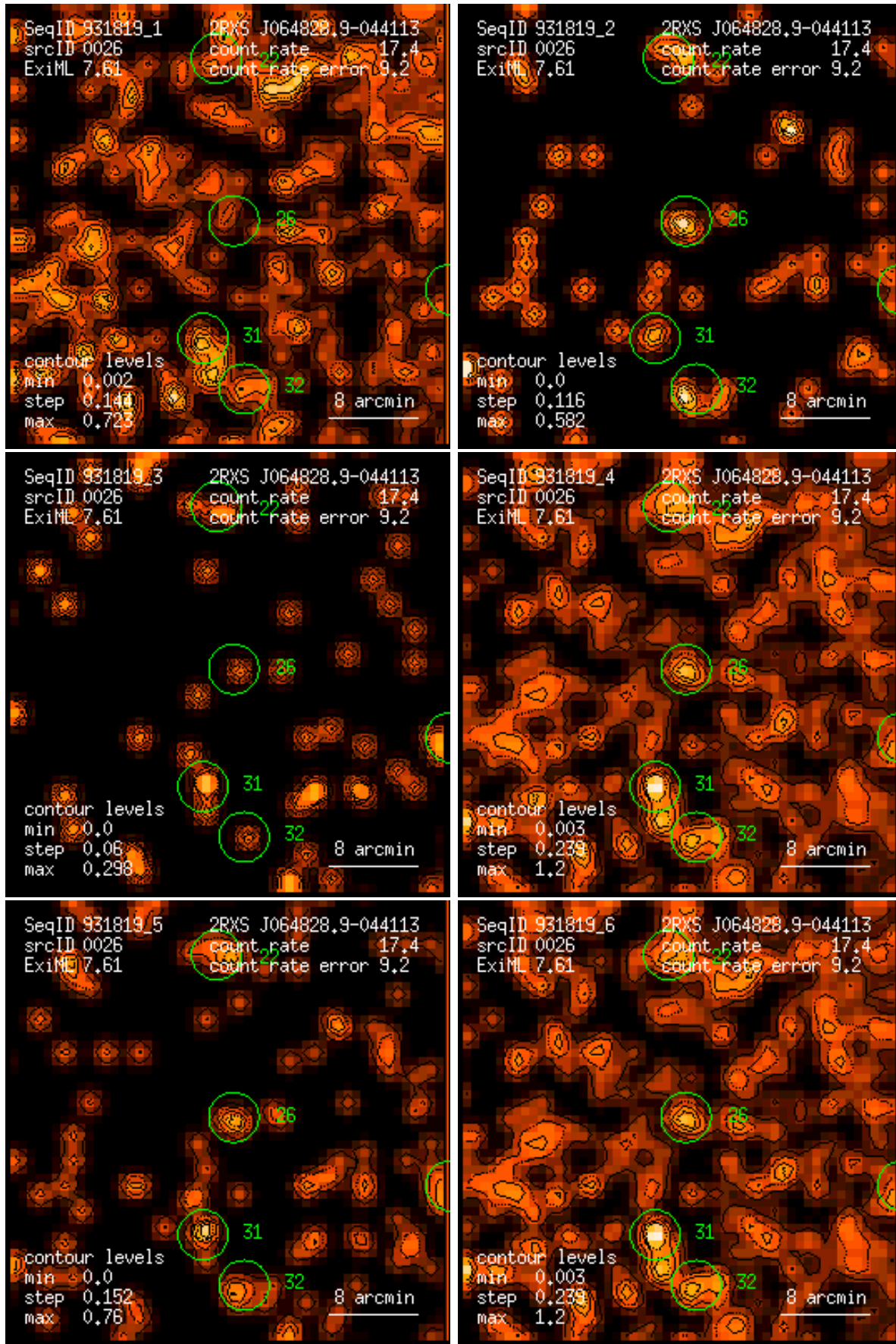
Figure 26: RASS 931819: detection 0026: band rate images, Gaussian filter: (1) PSPC channels 11 – 41, (2) 52 – 90, (3) 91 – 201, (4) 11 – 235, (5) 52 – 201, (6) 11 – 201. Broad band rates in counts/ks. Band rate contour levels in counts/ks/arcmin 2 .
