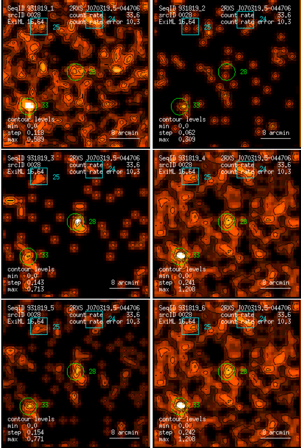
Figure 28: RASS 931819: detection 0028: band rate images, Gaussian filter: (1) PSPC channels 11 – 41, (2) 52 – 90, (3) 91 – 201, (4) 11 – 235, (5) 52 – 201, (6) 11 – 201. Broad band rates in counts/ks. Band rate contour levels in counts/ks/arcmin 2 .
