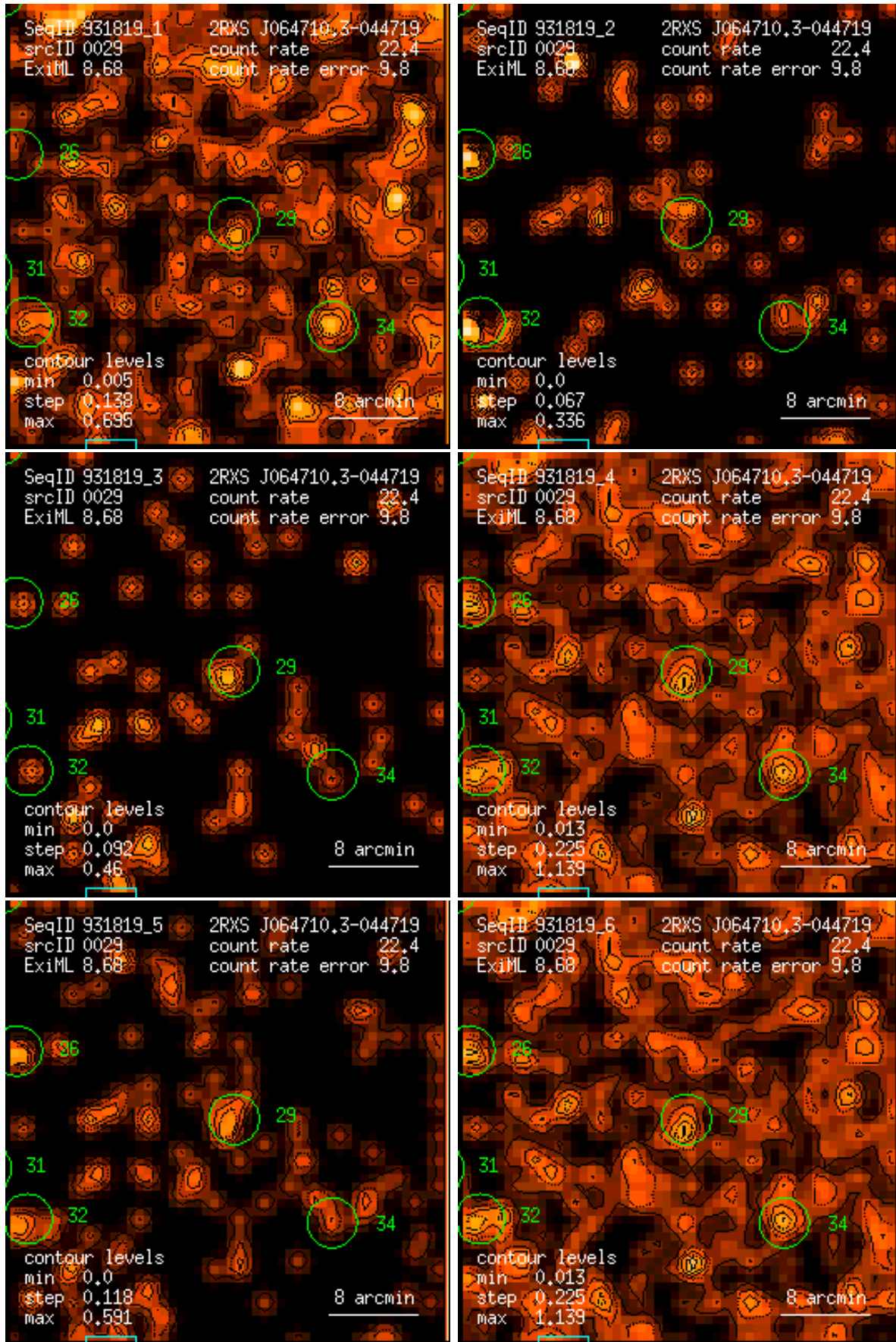
Figure 29: RASS 931819: detection 0029: band rate images, Gaussian filter: (1) PSPC channels 11 – 41, (2) 52 – 90, (3) 91 – 201, (4) 11 – 235, (5) 52 – 201, (6) 11 – 201. Broad band rates in counts/ks. Band rate contour levels in counts/ks/arcmin 2 .
