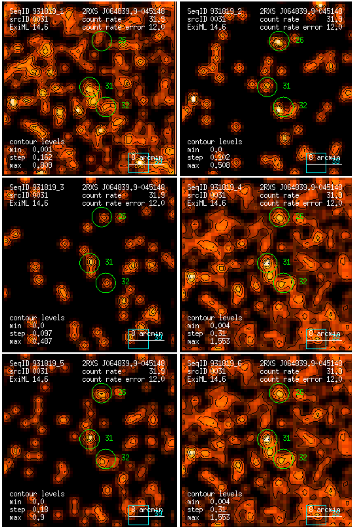
Figure 31: RASS 931819: detection 0031: band rate images, Gaussian filter: (1) PSPC channels 11 – 41, (2) 52 – 90, (3) 91 – 201, (4) 11 – 235, (5) 52 – 201, (6) 11 – 201. Broad band rates in counts/ks. Band rate contour levels in counts/ks/arcmin 2 .
