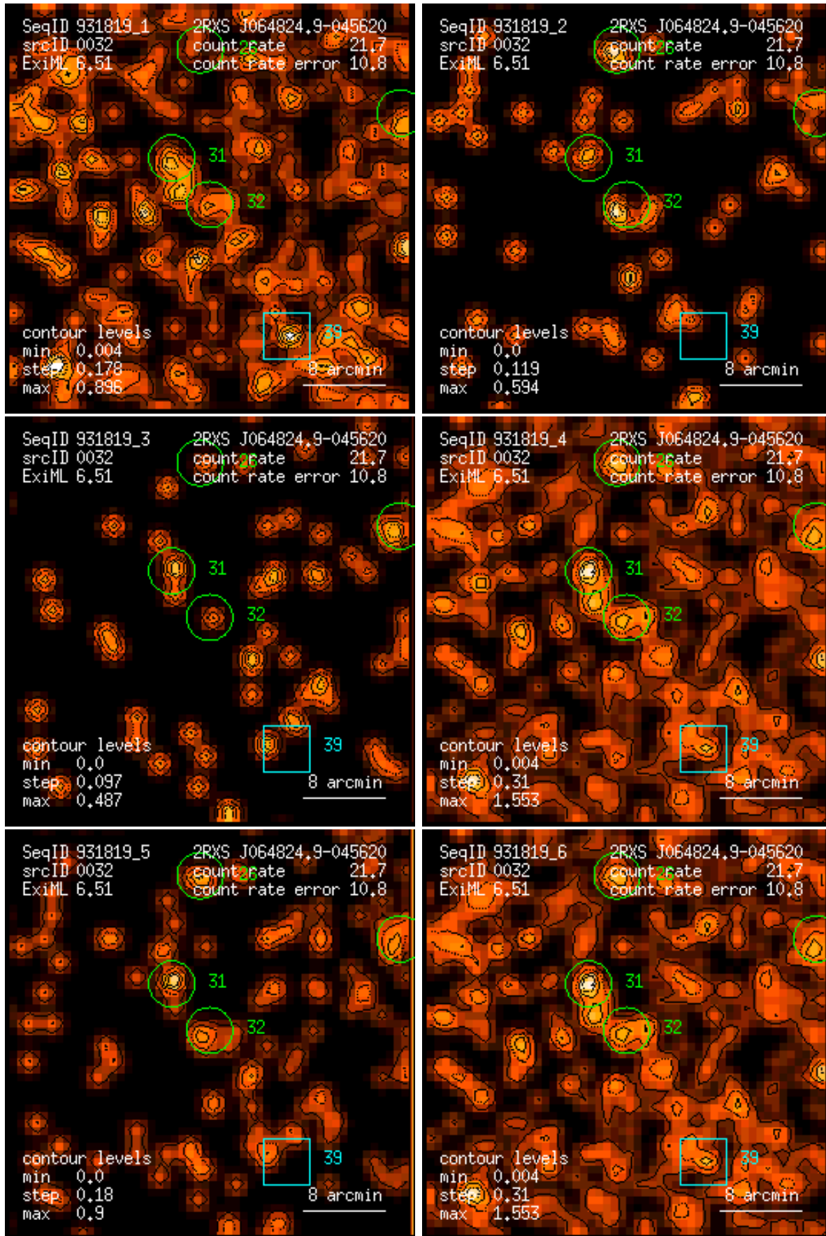
Figure 32: RASS 931819: detection 0032: band rate images, Gaussian filter: (1) PSPC channels 11 – 41, (2) 52 – 90, (3) 91 – 201, (4) 11 – 235, (5) 52 – 201, (6) 11 – 201. Broad band rates in counts/ks. Band rate contour levels in counts/ks/arcmin 2 .
