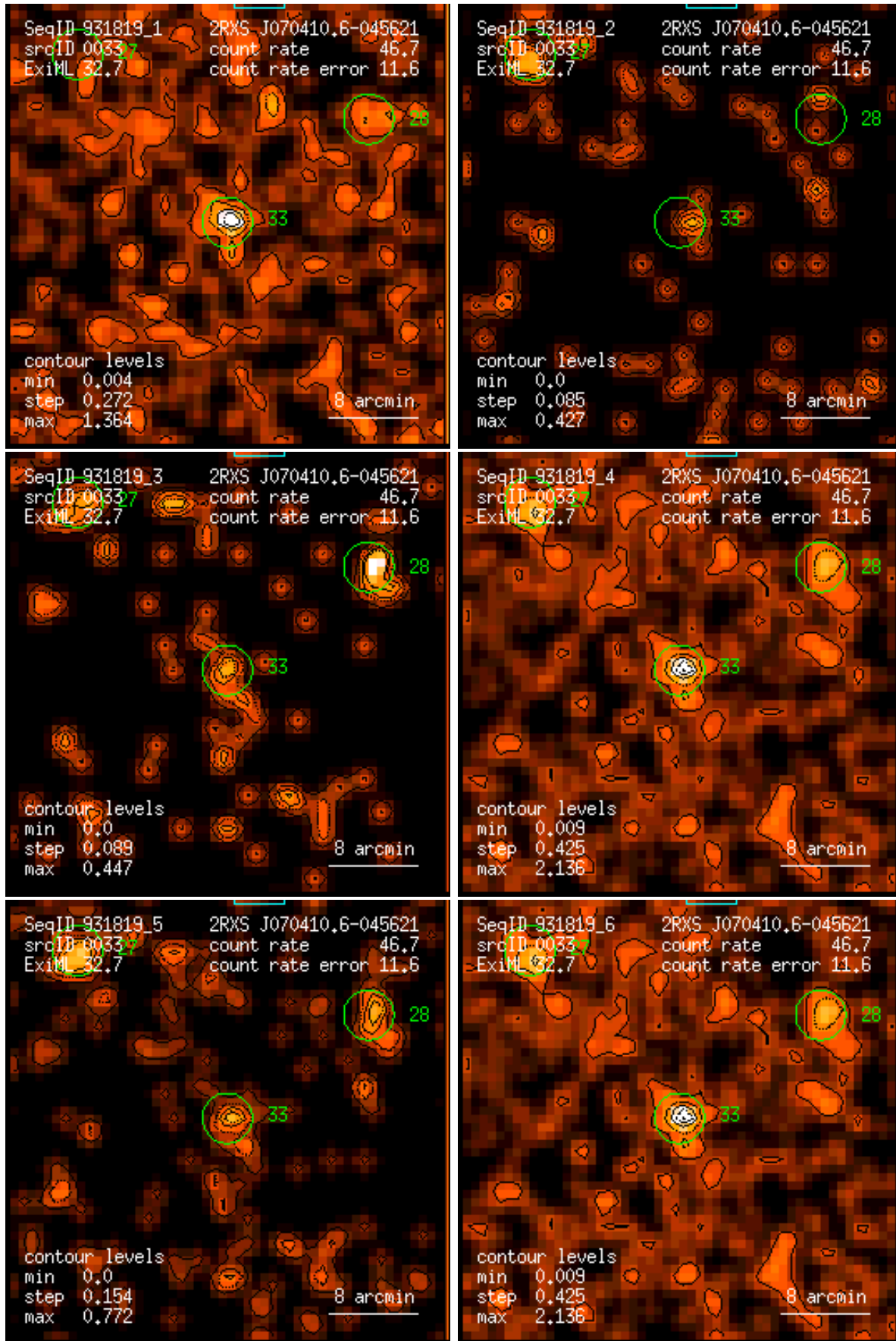
Figure 33: RASS 931819: detection 0033: band rate images, Gaussian filter: (1) PSPC channels 11 – 41, (2) 52 – 90, (3) 91 – 201, (4) 11 – 235, (5) 52 – 201, (6) 11 – 201. Broad band rates in counts/ks. Band rate contour levels in counts/ks/arcmin 2 .
