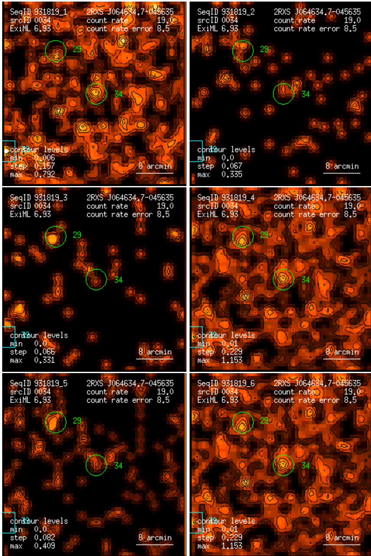
Figure 34: RASS 931819: detection 0034: band rate images, Gaussian filter: (1) PSPC channels 11 – 41, (2) 52 – 90, (3) 91 – 201, (4) 11 – 235, (5) 52 – 201, (6) 11 – 201. Broad band rates in counts/ks. Band rate contour levels in counts/ks/arcmin 2 .
