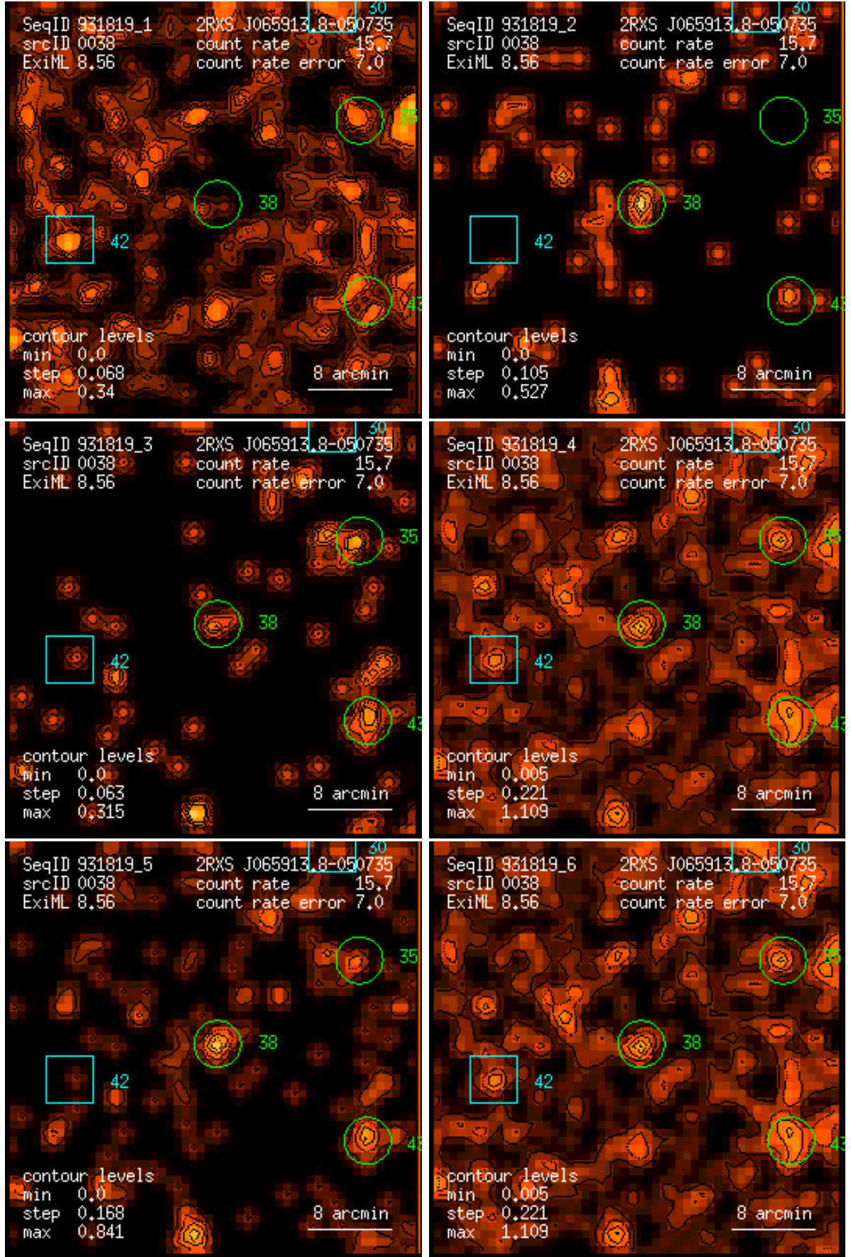
Figure 38: RASS 931819: detection 0038: band rate images, Gaussian filter: (1) PSPC channels 11 – 41, (2) 52 – 90, (3) 91 – 201, (4) 11 – 235, (5) 52 – 201, (6) 11 – 201. Broad band rates in counts/ks. Band rate contour levels in counts/ks/arcmin 2 .
