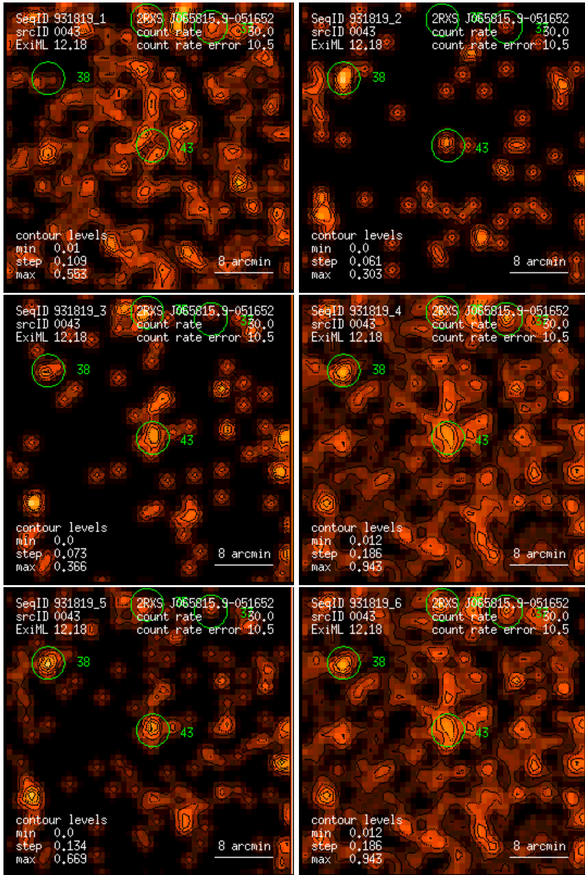
Figure 43: RASS 931819: detection 0043: band rate images, Gaussian filter: (1) PSPC channels 11 – 41, (2) 52 – 90, (3) 91 – 201, (4) 11 – 235, (5) 52 – 201, (6) 11 – 201. Broad band rates in counts/ks. Band rate contour levels in counts/ks/arcmin 2 .
