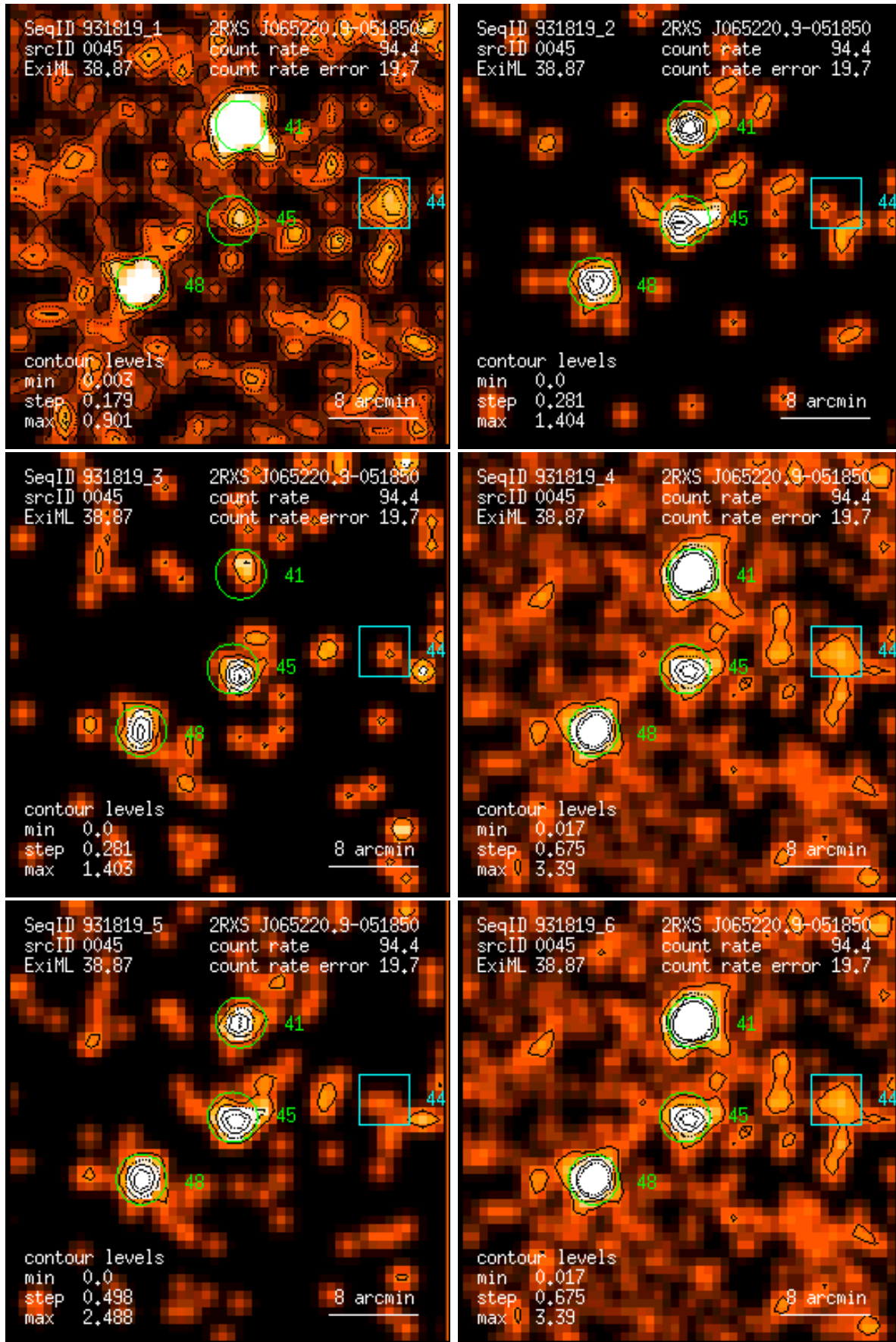
Figure 45: RASS 931819: detection 0045: band rate images, Gaussian filter: (1) PSPC channels 11 – 41, (2) 52 – 90, (3) 91 – 201, (4) 11 – 235, (5) 52 – 201, (6) 11 – 201. Broad band rates in counts/ks. Band rate contour levels in counts/ks/arcmin 2 .
