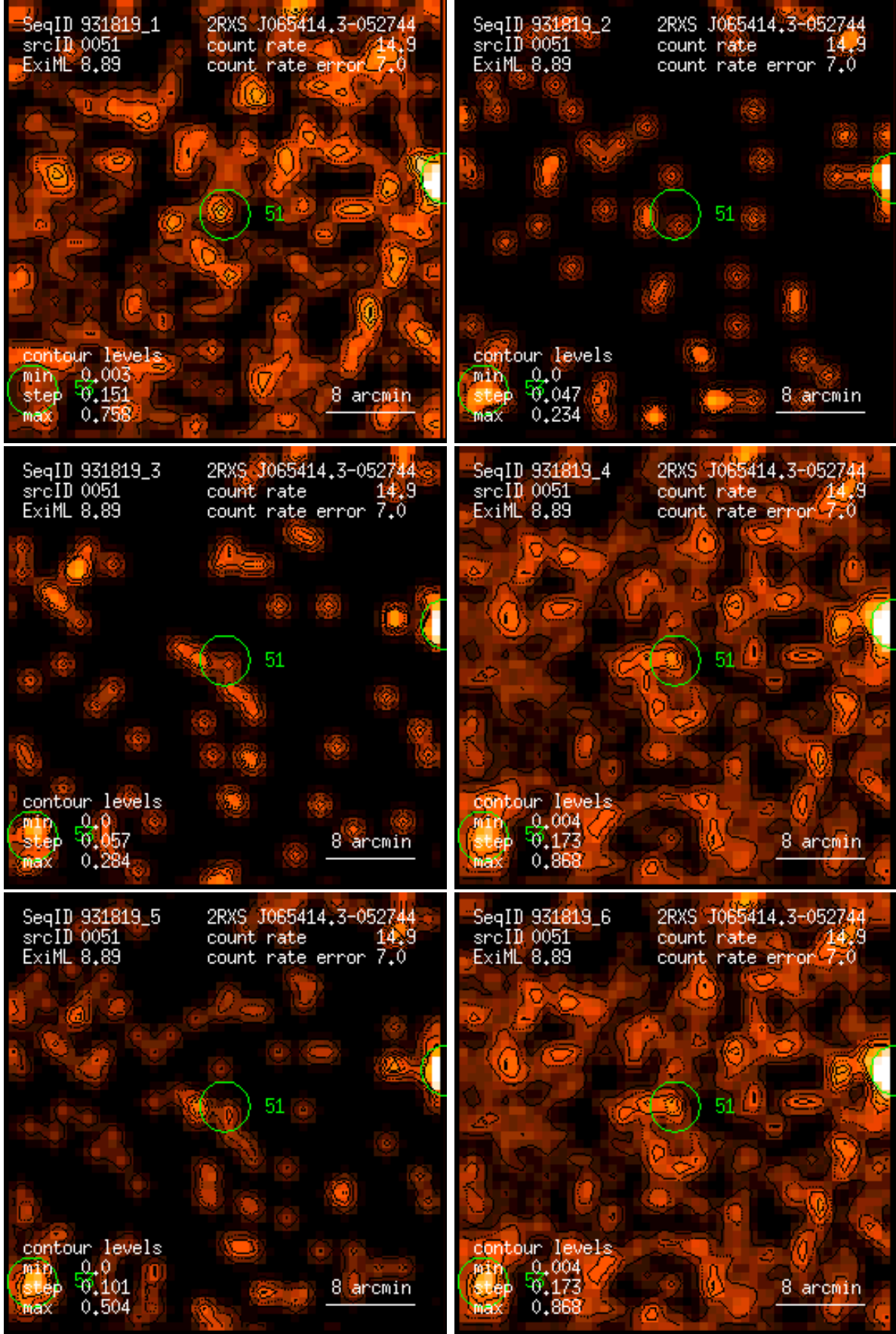
Figure 51: RASS 931819: detection 0051: band rate images, Gaussian filter: (1) PSPC channels 11 – 41, (2) 52 – 90, (3) 91 – 201, (4) 11 – 235, (5) 52 – 201, (6) 11 – 201. Broad band rates in counts/ks. Band rate contour levels in counts/ks/arcmin 2 .
