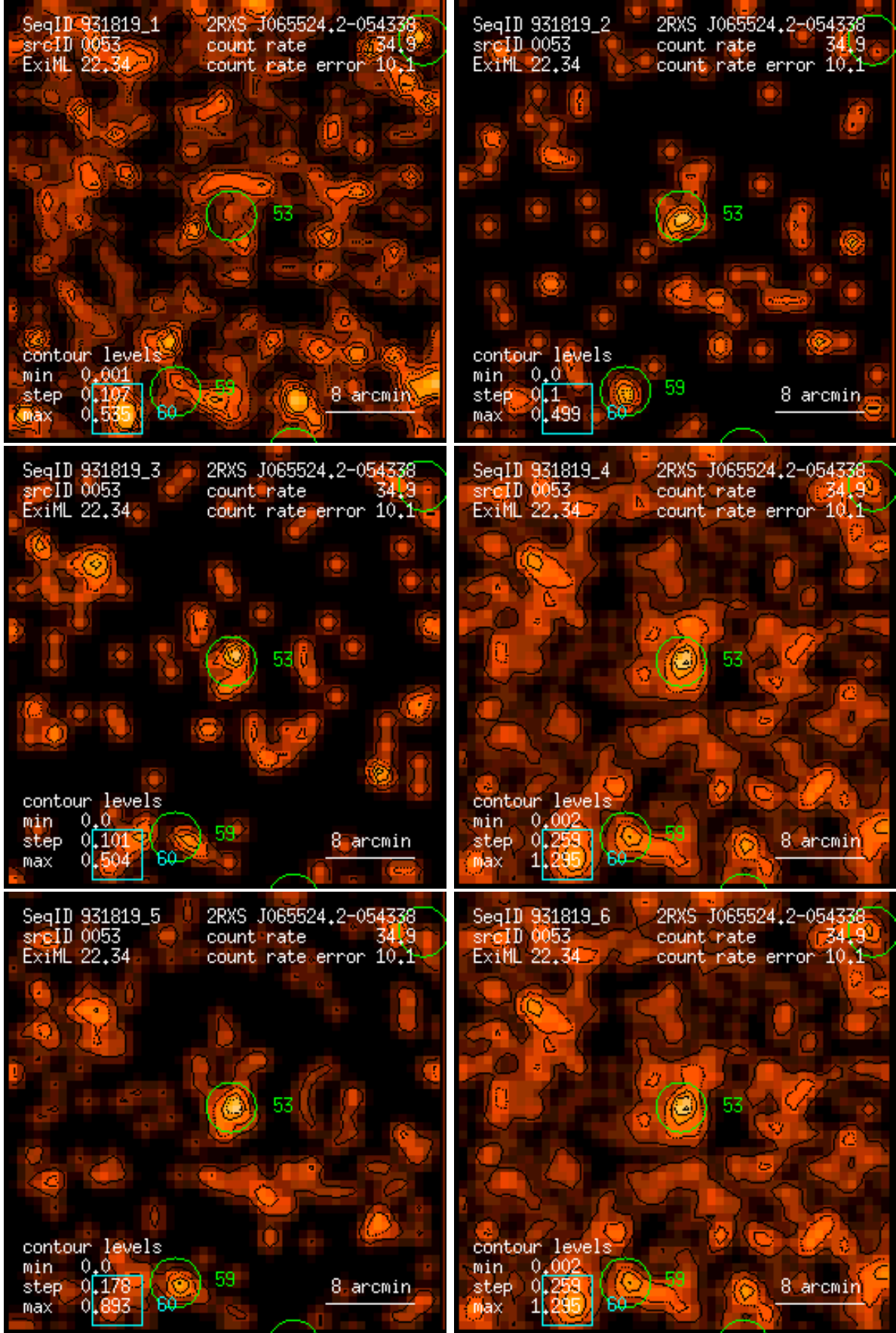
Figure 53: RASS 931819: detection 0053: band rate images, Gaussian filter: (1) PSPC channels 11 – 41, (2) 52 – 90, (3) 91 – 201, (4) 11 – 235, (5) 52 – 201, (6) 11 – 201. Broad band rates in counts/ks. Band rate contour levels in counts/ks/arcmin 2 .
