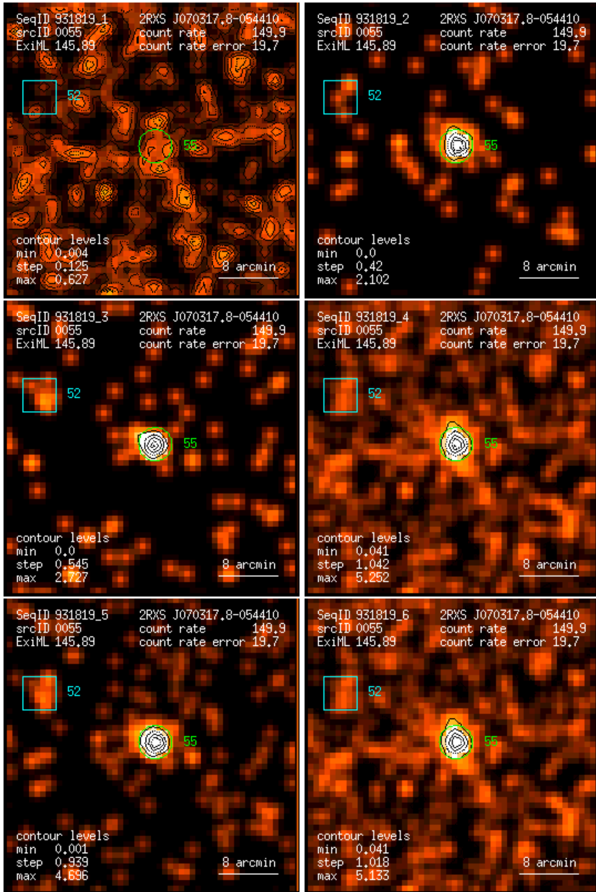
Figure 55: RASS 931819: detection 0055: band rate images, Gaussian filter: (1) PSPC channels 11 – 41, (2) 52 – 90, (3) 91 – 201, (4) 11 – 235, (5) 52 – 201, (6) 11 – 201. Broad band rates in counts/ks. Band rate contour levels in counts/ks/arcmin 2 .
