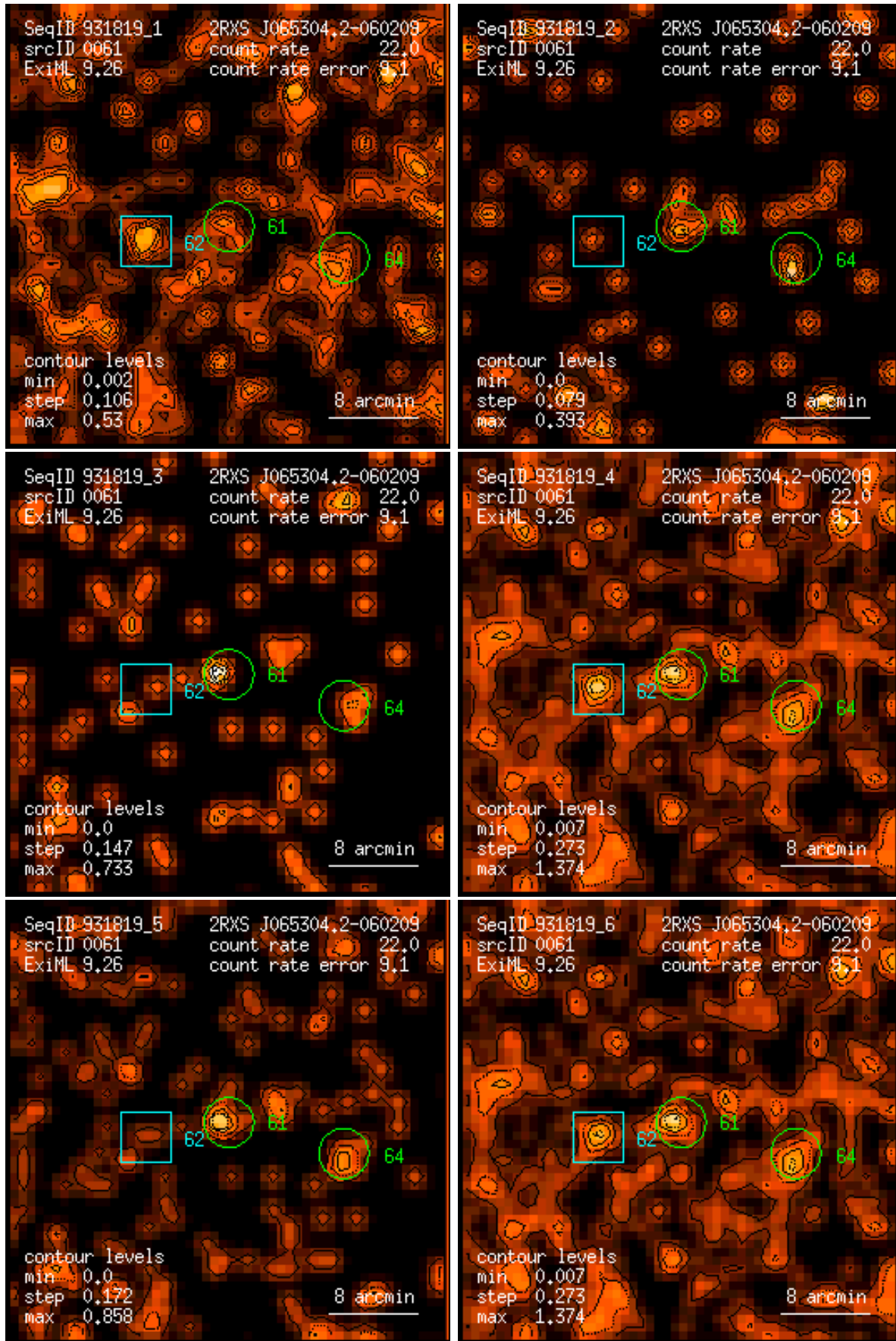
Figure 61: RASS 931819: detection 0061: band rate images, Gaussian filter: (1) PSPC channels 11 – 41, (2) 52 – 90, (3) 91 – 201, (4) 11 – 235, (5) 52 – 201, (6) 11 – 201. Broad band rates in counts/ks. Band rate contour levels in counts/ks/arcmin 2 .
