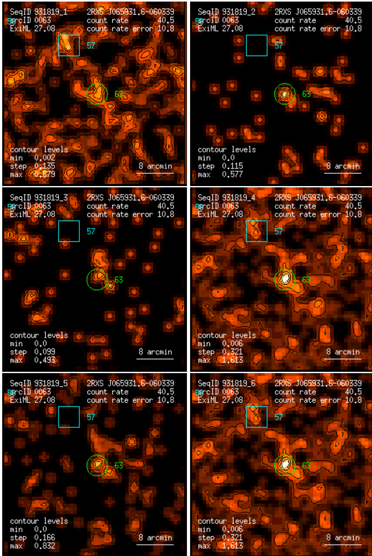
Figure 63: RASS 931819: detection 0063: band rate images, Gaussian filter: (1) PSPC channels 11 – 41, (2) 52 – 90, (3) 91 – 201, (4) 11 – 235, (5) 52 – 201, (6) 11 – 201. Broad band rates in counts/ks. Band rate contour levels in counts/ks/arcmin 2 .
