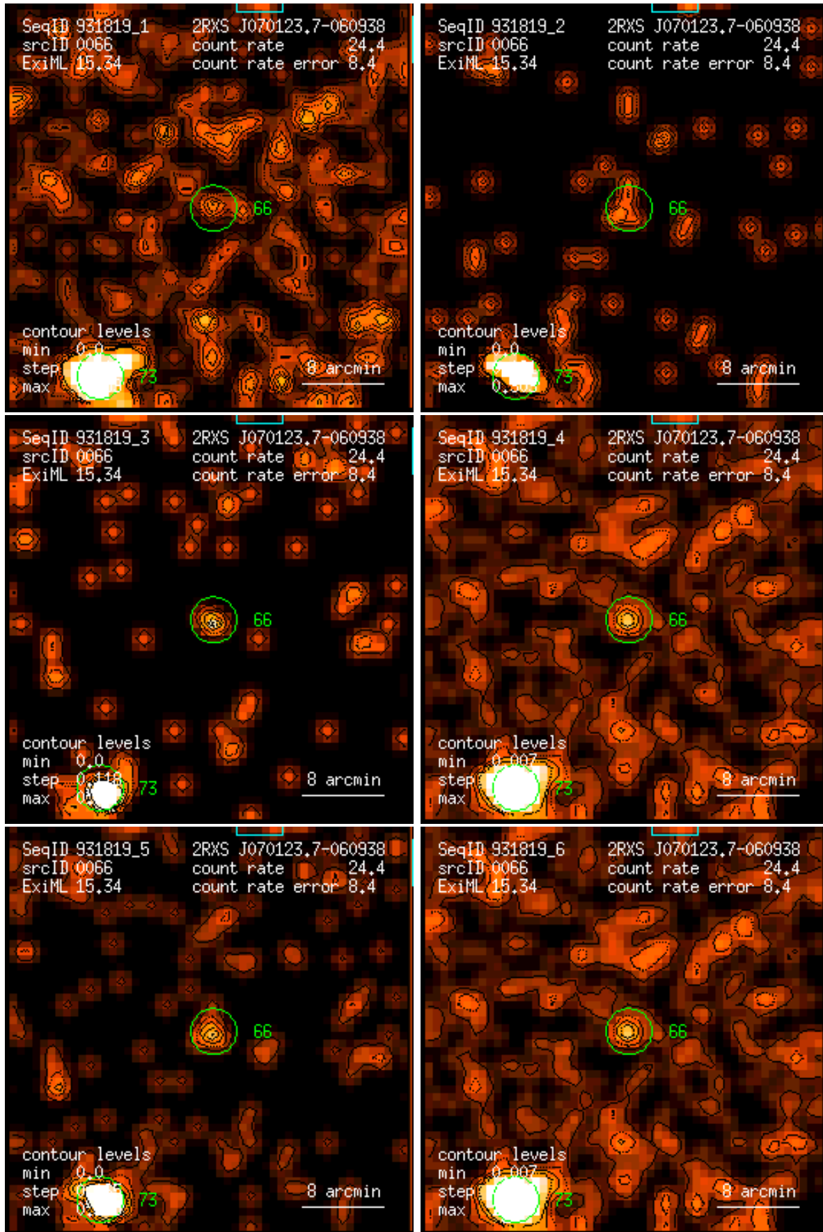
Figure 66: RASS 931819: detection 0066: band rate images, Gaussian filter: (1) PSPC channels 11 – 41, (2) 52 – 90, (3) 91 – 201, (4) 11 – 235, (5) 52 – 201, (6) 11 – 201. Broad band rates in counts/ks. Band rate contour levels in counts/ks/arcmin 2 .
