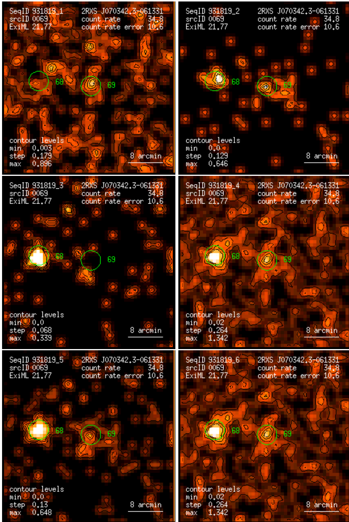
Figure 69: RASS 931819: detection 0069: band rate images, Gaussian filter: (1) PSPC channels 11 – 41, (2) 52 – 90, (3) 91 – 201, (4) 11 – 235, (5) 52 – 201, (6) 11 – 201. Broad band rates in counts/ks. Band rate contour levels in counts/ks/arcmin 2 .
