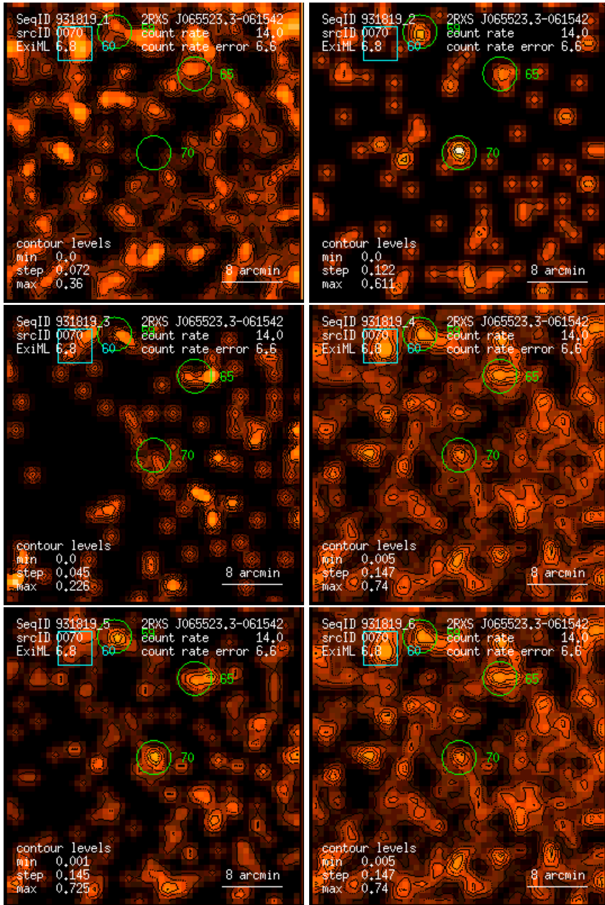
Figure 70: RASS 931819: detection 0070: band rate images, Gaussian filter: (1) PSPC channels 11 – 41, (2) 52 – 90, (3) 91 – 201, (4) 11 – 235, (5) 52 – 201, (6) 11 – 201. Broad band rates in counts/ks. Band rate contour levels in counts/ks/arcmin 2 .
