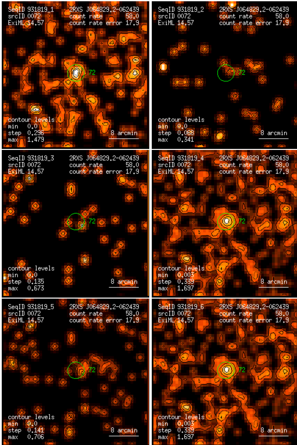
Figure 72: RASS 931819: detection 0072: band rate images, Gaussian filter: (1) PSPC channels 11 – 41, (2) 52 – 90, (3) 91 – 201, (4) 11 – 235, (5) 52 – 201, (6) 11 – 201. Broad band rates in counts/ks. Band rate contour levels in counts/ks/arcmin 2 .
