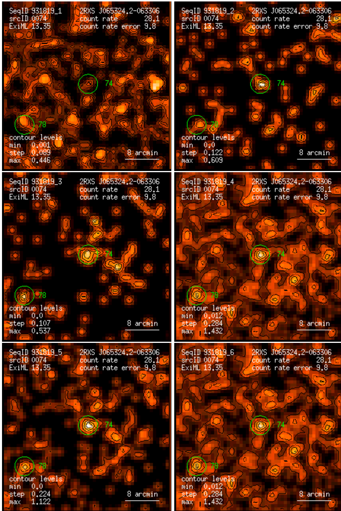
Figure 74: RASS 931819: detection 0074: band rate images, Gaussian filter: (1) PSPC channels 11 – 41, (2) 52 – 90, (3) 91 – 201, (4) 11 – 235, (5) 52 – 201, (6) 11 – 201. Broad band rates in counts/ks. Band rate contour levels in counts/ks/arcmin 2 .
