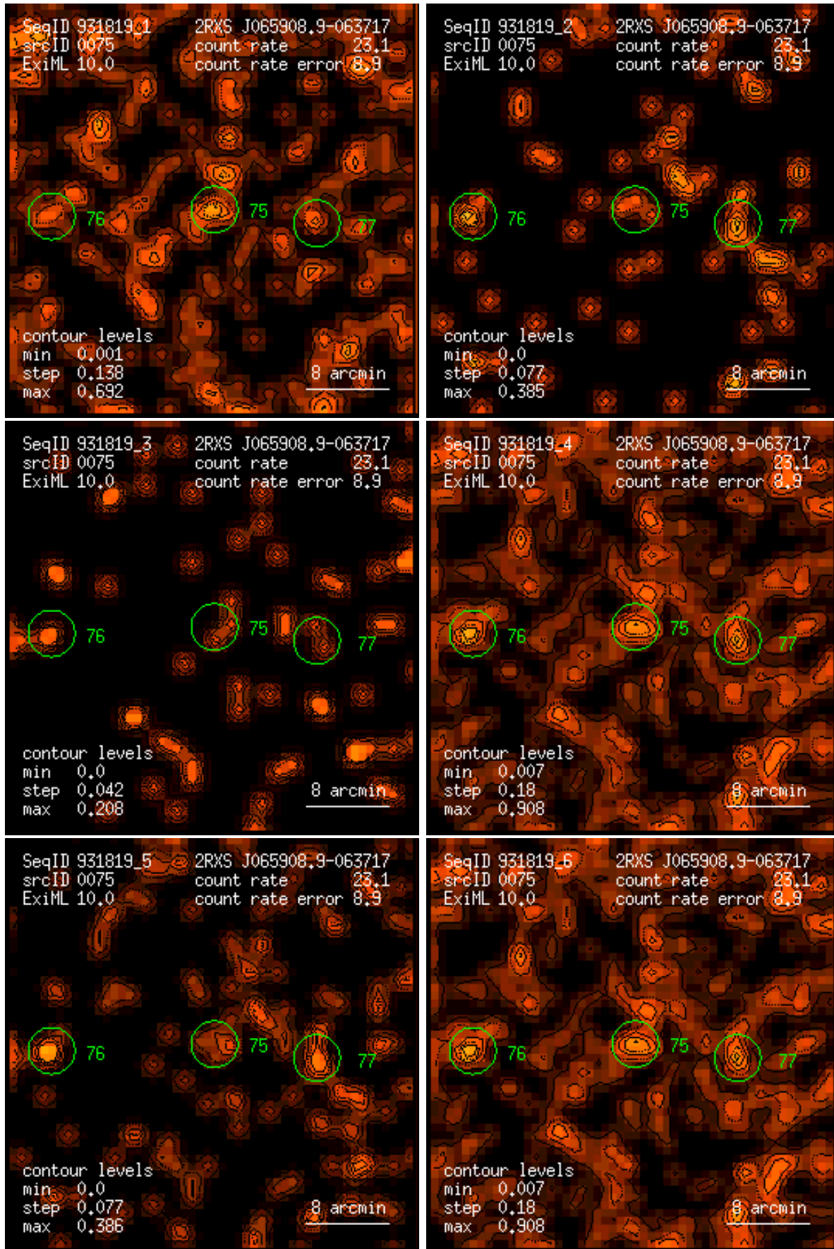
Figure 75: RASS 931819: detection 0075: band rate images, Gaussian filter: (1) PSPC channels 11 – 41, (2) 52 – 90, (3) 91 – 201, (4) 11 – 235, (5) 52 – 201, (6) 11 – 201. Broad band rates in counts/ks. Band rate contour levels in counts/ks/arcmin 2 .
