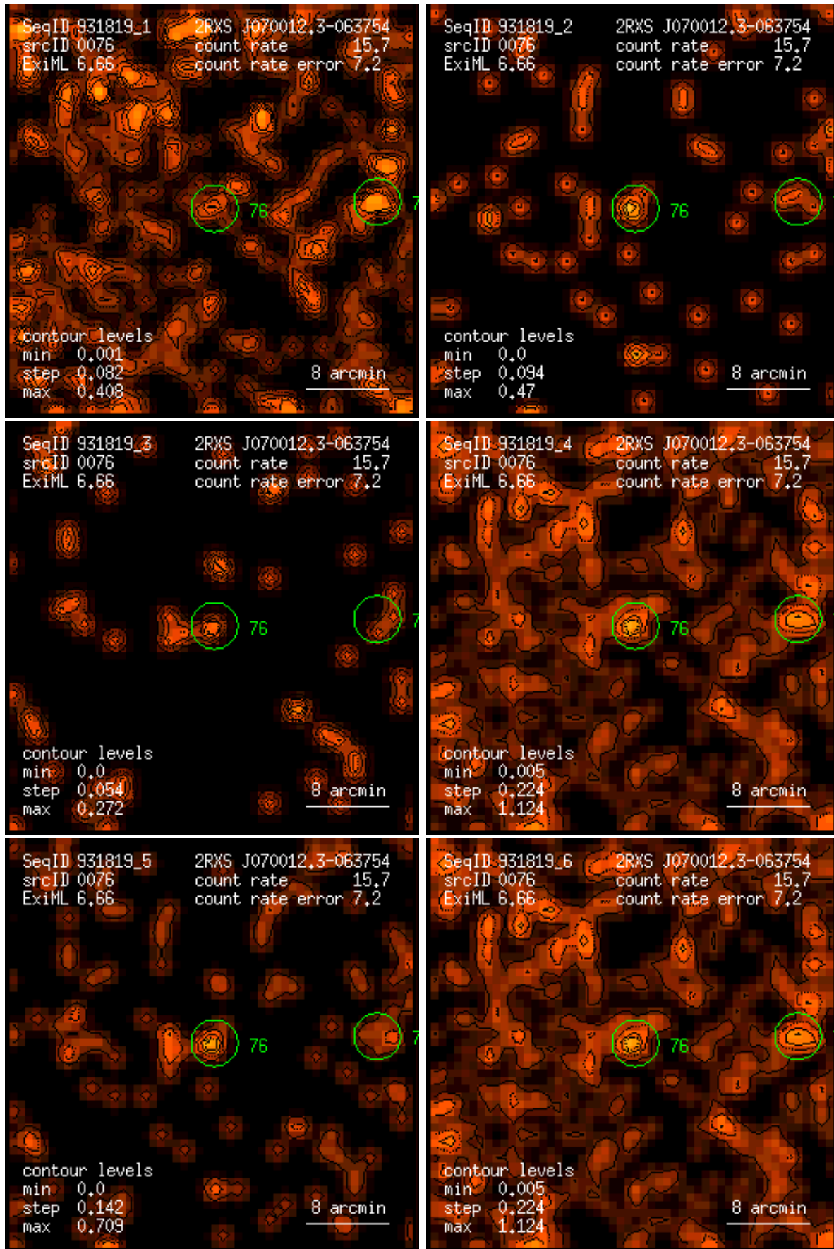
Figure 76: RASS 931819: detection 0076: band rate images, Gaussian filter: (1) PSPC channels 11 – 41, (2) 52 – 90, (3) 91 – 201, (4) 11 – 235, (5) 52 – 201, (6) 11 – 201. Broad band rates in counts/ks. Band rate contour levels in counts/ks/arcmin 2 .
