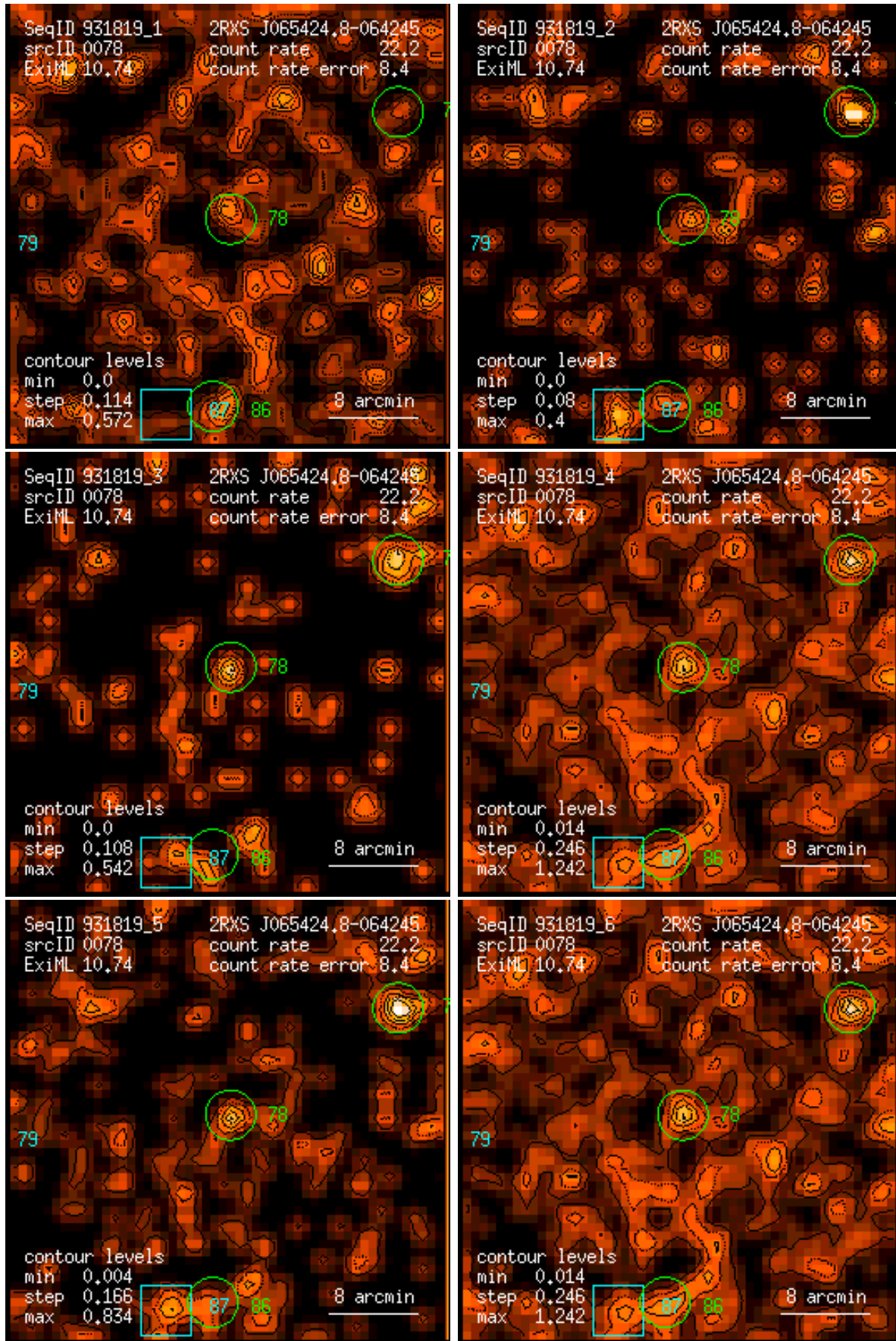
Figure 78: RASS 931819: detection 0078: band rate images, Gaussian filter: (1) PSPC channels 11 – 41, (2) 52 – 90, (3) 91 – 201, (4) 11 – 235, (5) 52 – 201, (6) 11 – 201. Broad band rates in counts/ks. Band rate contour levels in counts/ks/arcmin 2 .
