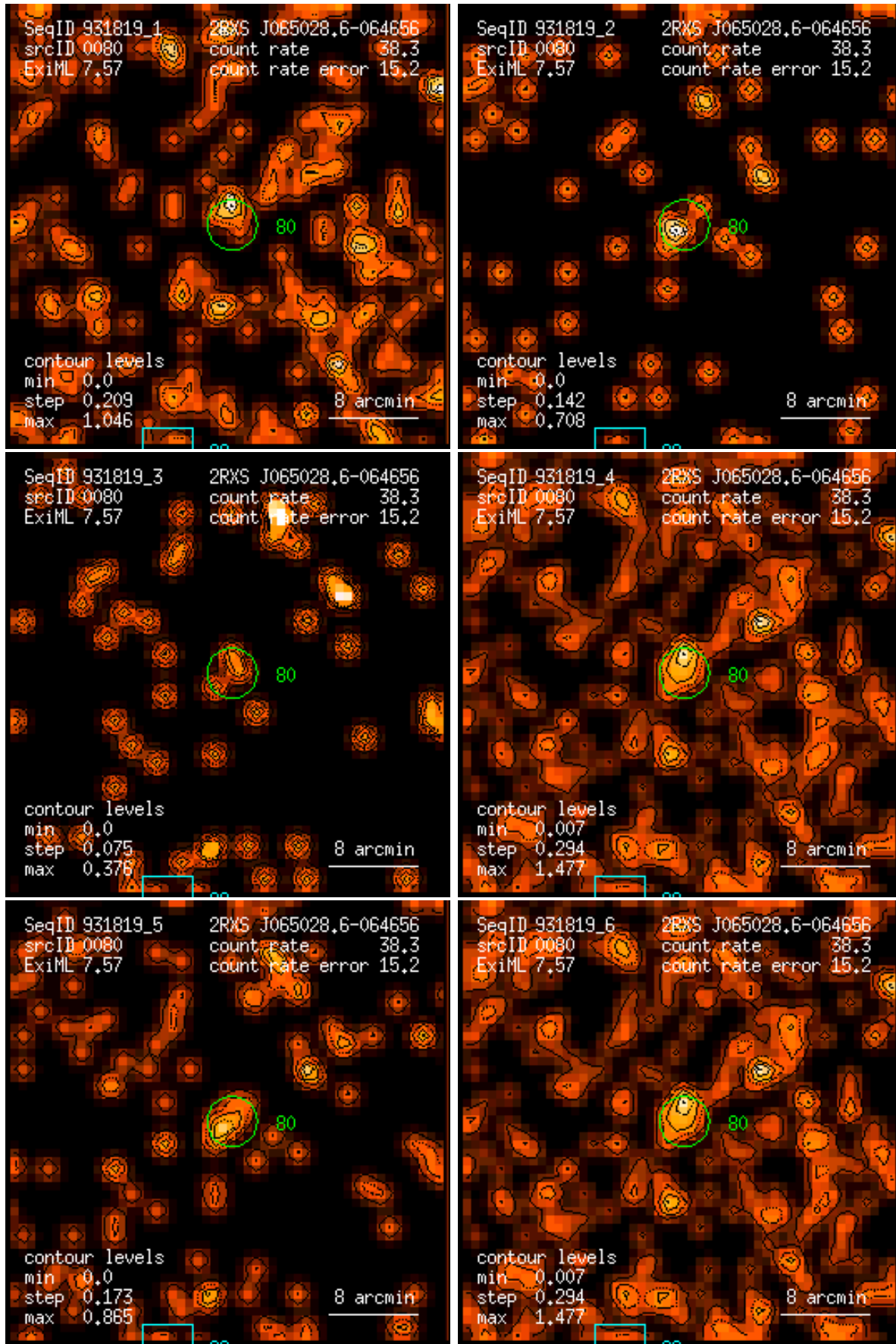
Figure 80: RASS 931819: detection 0080: band rate images, Gaussian filter: (1) PSPC channels 11 – 41, (2) 52 – 90, (3) 91 – 201, (4) 11 – 235, (5) 52 – 201, (6) 11 – 201. Broad band rates in counts/ks. Band rate contour levels in counts/ks/arcmin 2 .
