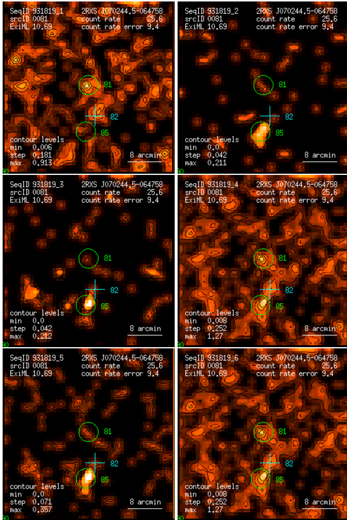
Figure 81: RASS 931819: detection 0081: band rate images, Gaussian filter: (1) PSPC channels 11 – 41, (2) 52 – 90, (3) 91 – 201, (4) 11 – 235, (5) 52 – 201, (6) 11 – 201. Broad band rates in counts/ks. Band rate contour levels in counts/ks/arcmin 2 .
