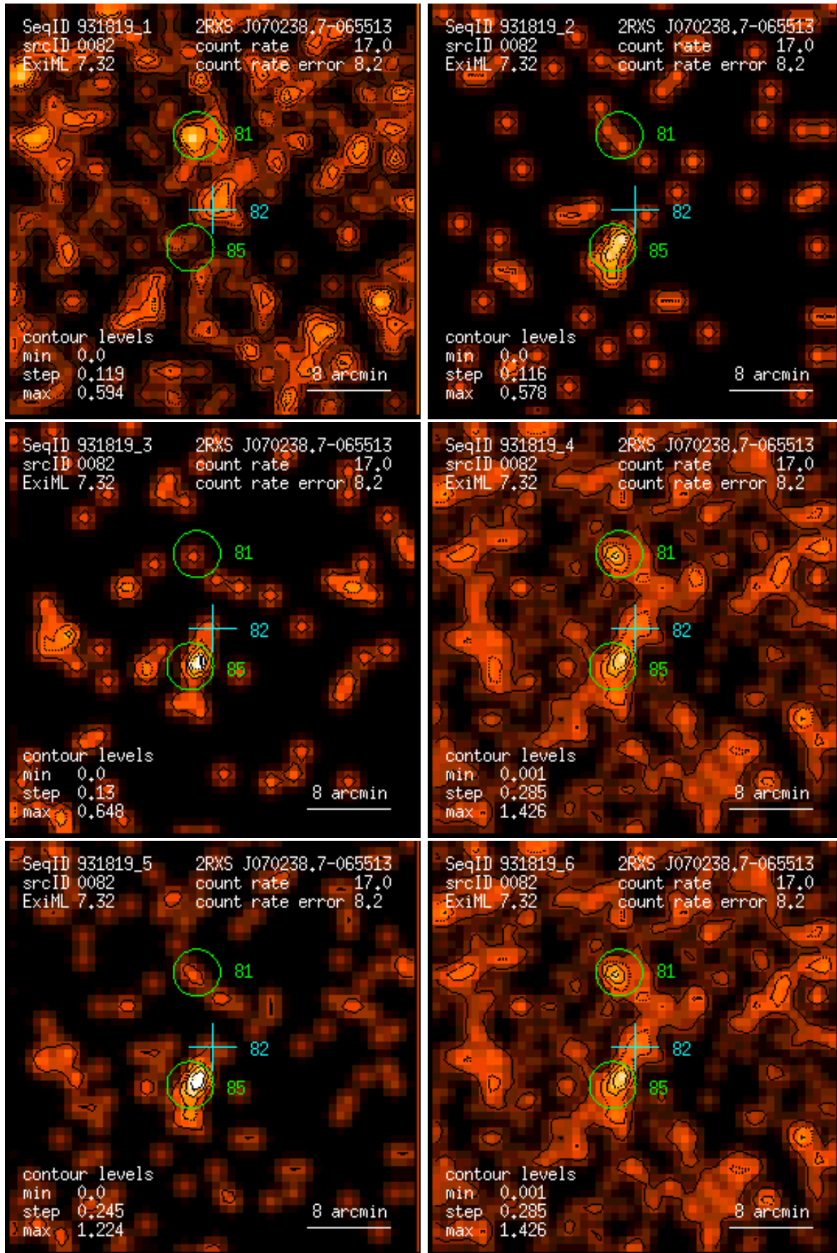
Figure 82: RASS 931819: detection 0082: band rate images, Gaussian filter: (1) PSPC channels 11 – 41, (2) 52 – 90, (3) 91 – 201, (4) 11 – 235, (5) 52 – 201, (6) 11 – 201. Broad band rates in counts/ks. Band rate contour levels in counts/ks/arcmin 2 .
