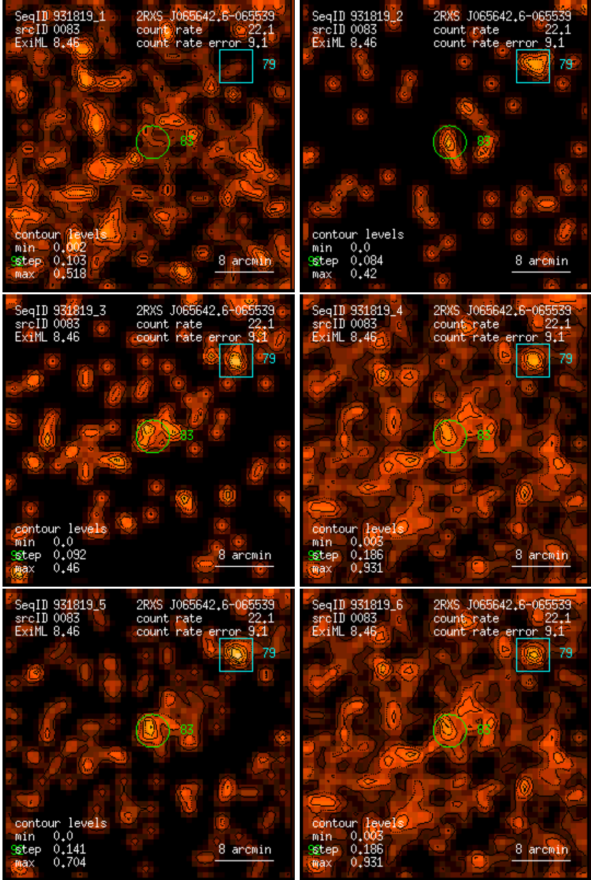
Figure 83: RASS 931819: detection 0083: band rate images, Gaussian filter: (1) PSPC channels 11 – 41, (2) 52 – 90, (3) 91 – 201, (4) 11 – 235, (5) 52 – 201, (6) 11 – 201. Broad band rates in counts/ks. Band rate contour levels in counts/ks/arcmin 2 .
