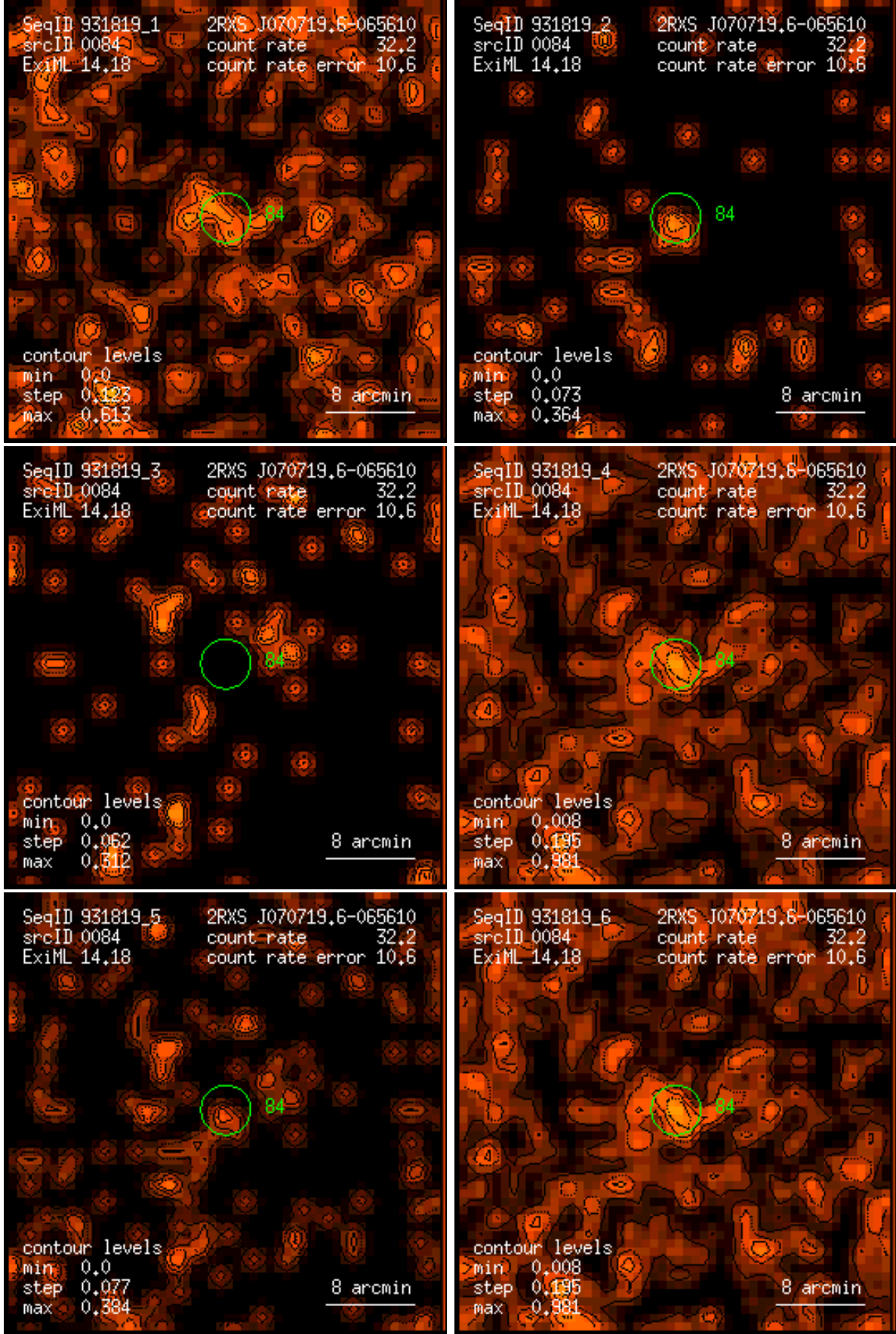
Figure 84: RASS 931819: detection 0084: band rate images, Gaussian filter: (1) PSPC channels 11 – 41, (2) 52 – 90, (3) 91 – 201, (4) 11 – 235, (5) 52 – 201, (6) 11 – 201. Broad band rates in counts/ks. Band rate contour levels in counts/ks/arcmin 2 .
