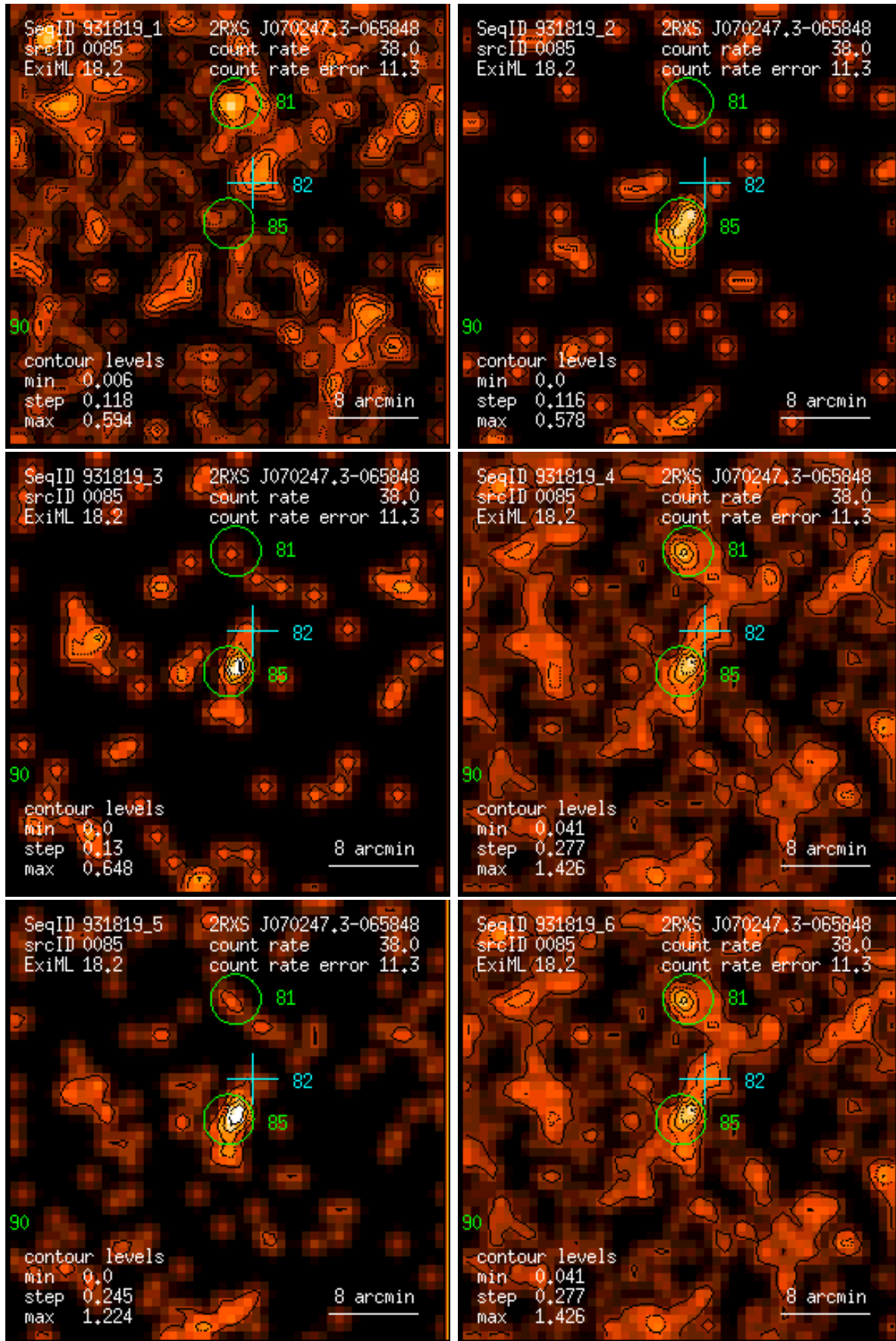
Figure 85: RASS 931819: detection 0085: band rate images, Gaussian filter: (1) PSPC channels 11 – 41, (2) 52 – 90, (3) 91 – 201, (4) 11 – 235, (5) 52 – 201, (6) 11 – 201. Broad band rates in counts/ks. Band rate contour levels in counts/ks/arcmin 2 .
