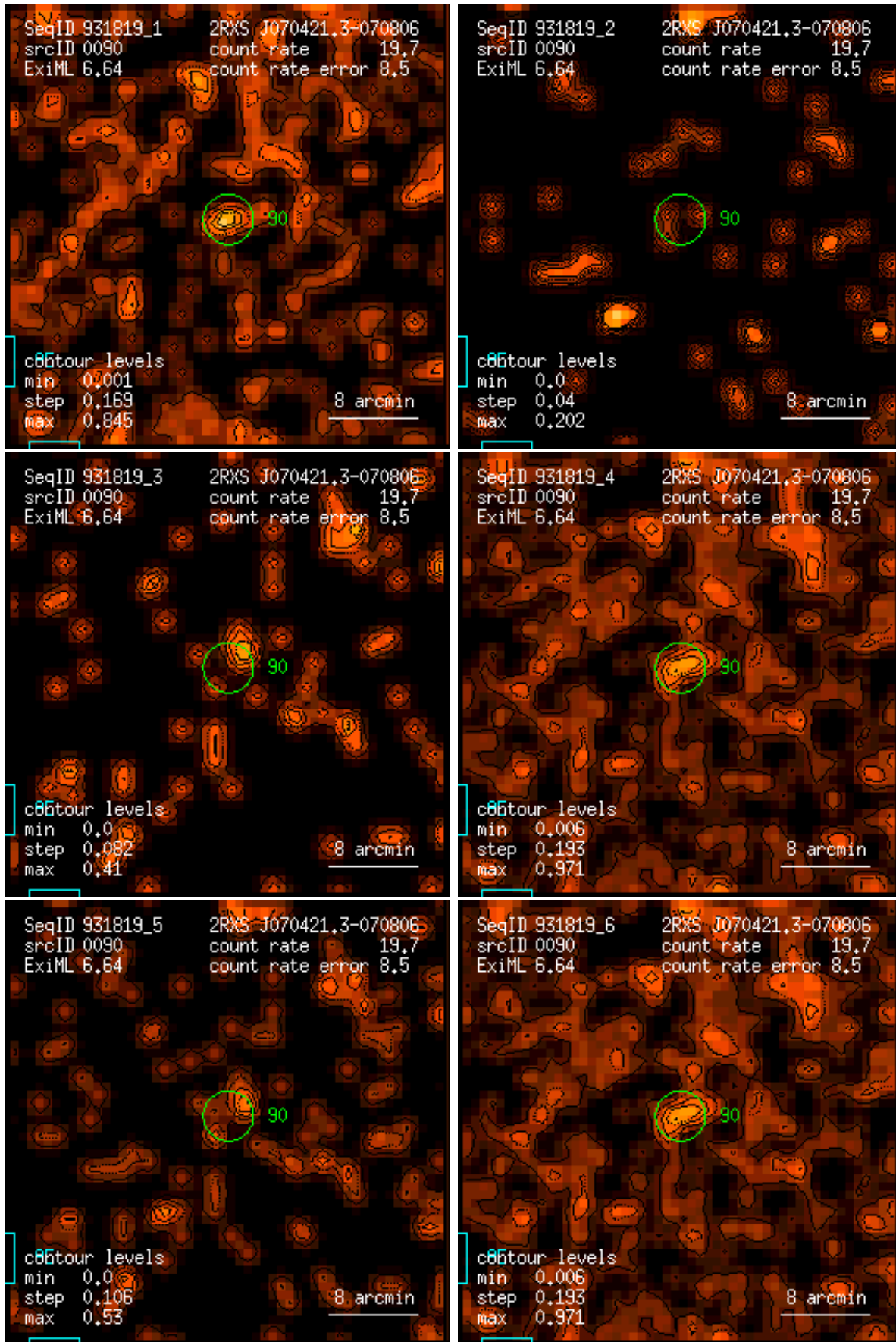
Figure 90: RASS 931819: detection 0090: band rate images, Gaussian filter: (1) PSPC channels 11 – 41, (2) 52 – 90, (3) 91 – 201, (4) 11 – 235, (5) 52 – 201, (6) 11 – 201. Broad band rates in counts/ks. Band rate contour levels in counts/ks/arcmin 2 .
