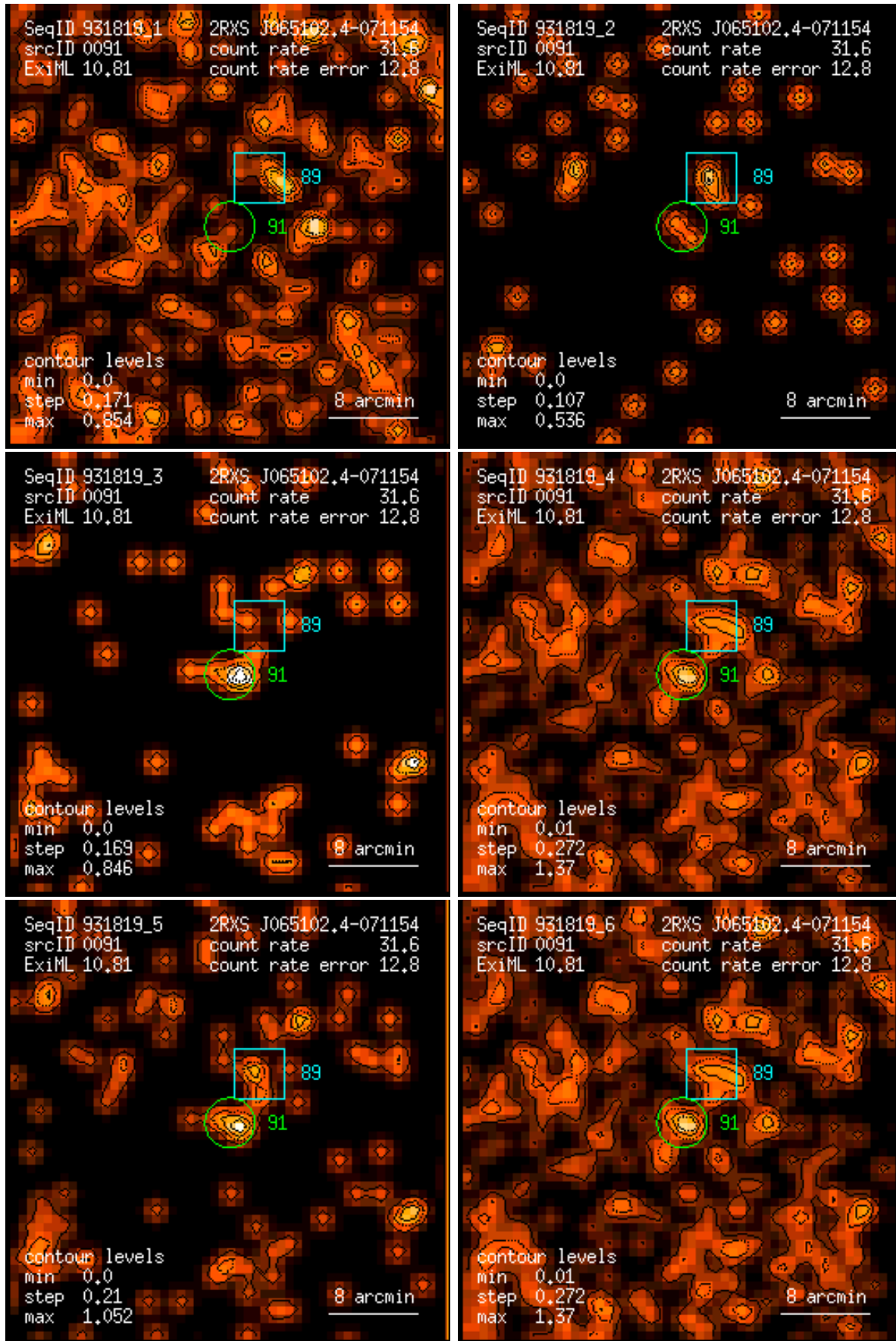
Figure 91: RASS 931819: detection 0091: band rate images, Gaussian filter: (1) PSPC channels 11 – 41, (2) 52 – 90, (3) 91 – 201, (4) 11 – 235, (5) 52 – 201, (6) 11 – 201. Broad band rates in counts/ks. Band rate contour levels in counts/ks/arcmin 2 .
