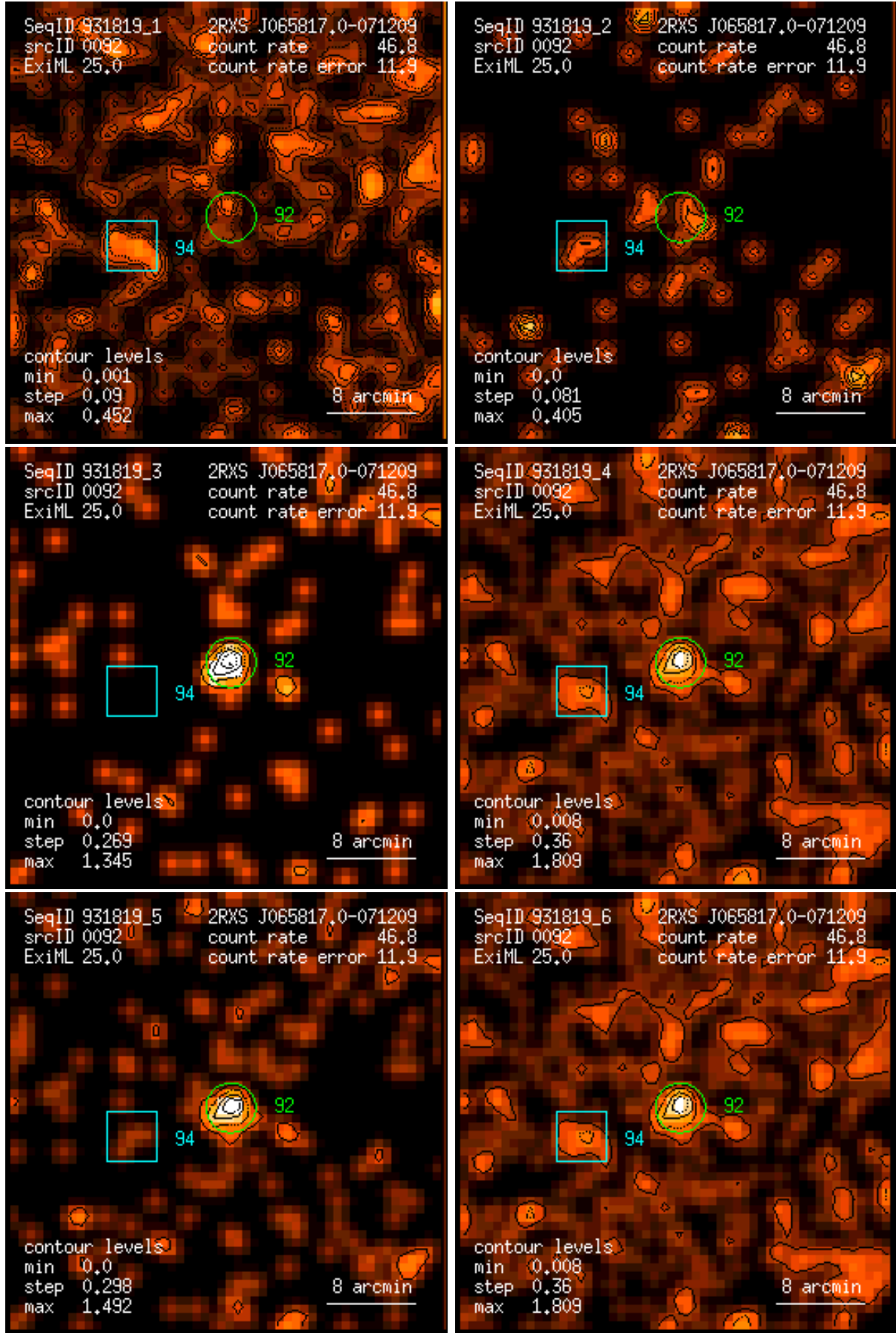
Figure 92: RASS 931819: detection 0092: band rate images, Gaussian filter: (1) PSPC channels 11 – 41, (2) 52 – 90, (3) 91 – 201, (4) 11 – 235, (5) 52 – 201, (6) 11 – 201. Broad band rates in counts/ks. Band rate contour levels in counts/ks/arcmin 2 .
