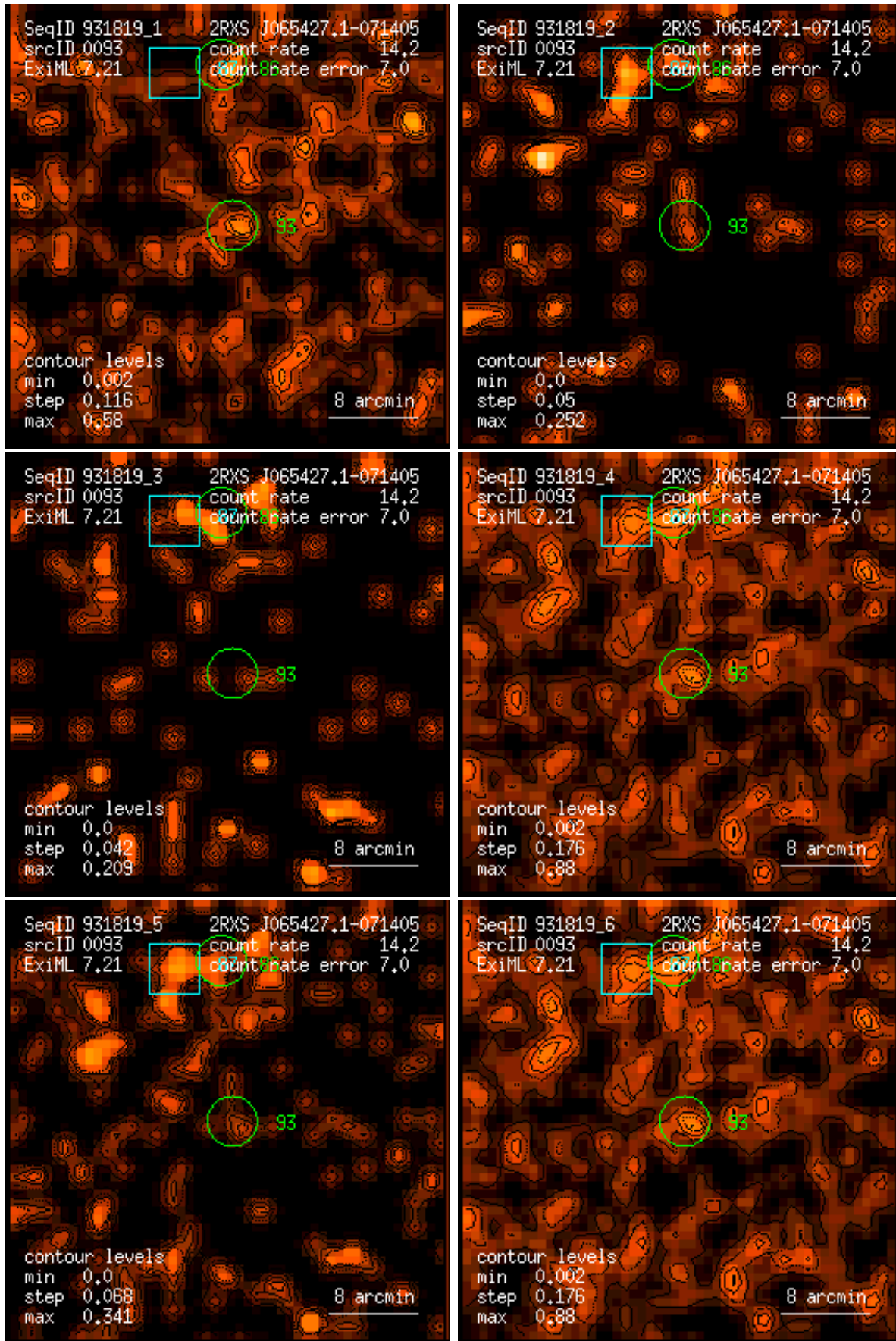
Figure 93: RASS 931819: detection 0093: band rate images, Gaussian filter: (1) PSPC channels 11 – 41, (2) 52 – 90, (3) 91 – 201, (4) 11 – 235, (5) 52 – 201, (6) 11 – 201. Broad band rates in counts/ks. Band rate contour levels in counts/ks/arcmin 2 .
